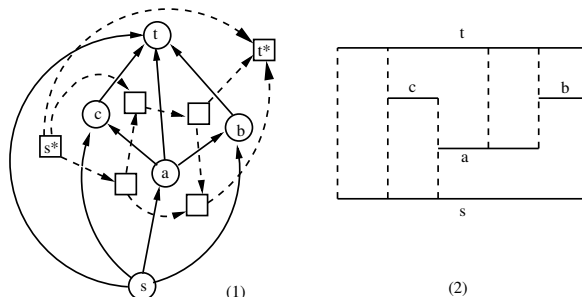
■ Figure 1 (1) An st -graph G and its st -dual graph G^* ; (2) A VR of G .
