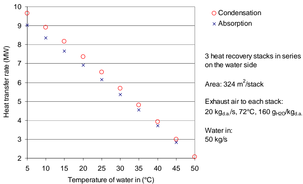
Fig. 2. Heat transfer rates for an example heat recovery system by using mass transfer equations for condensation and absorption: average difference 6 %.
