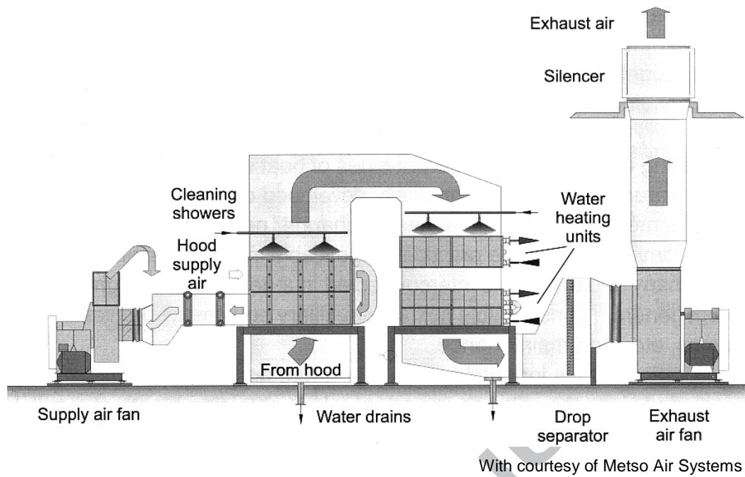
Fig. 1. Modern heat recovery stack of a paper machine dryer section.
