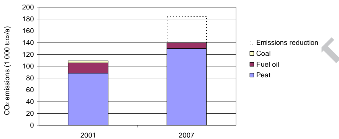
Fig. 6. Carbon dioxide emissions from the case mill power plant in 2001 and 2007 including estimated emissions reduction.
