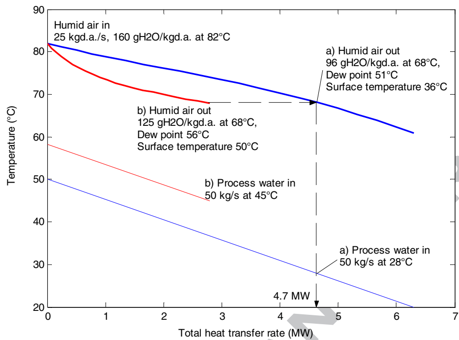
Fig. 3. The humidity of air after each match (here case a or b) at a certain temperature interval of the air (here 82 to 68°C) is unique if condensation occurs.
