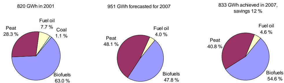
Fig. 5. Fuel use in 2001 and the forecast and actual fuel uses in the case mill in 2007.
