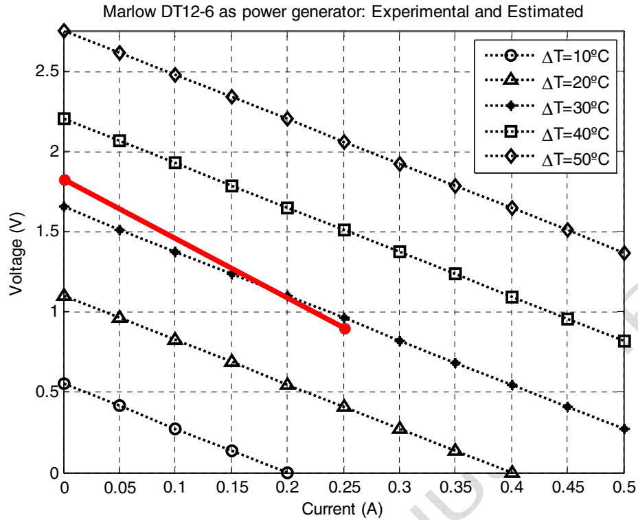
Figure 4: Estimated response for T=35^{\circ}\text{C}
