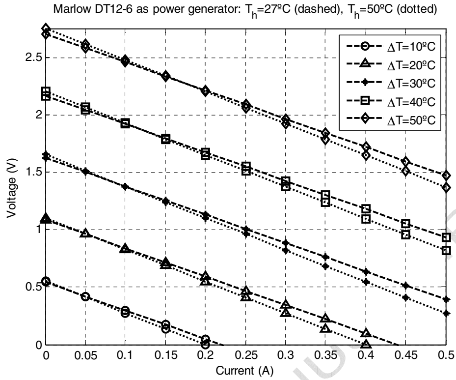
Figure 3: Estimated response for T_h=27^\circ\text{C} and T_h=50^\circ\text{C}
