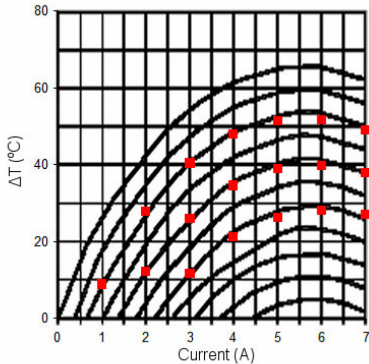
Figure 2: Simulated dots in a layer over the original Performance Curves of Marlow DT 12-6 [2]
