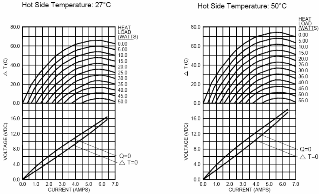
Figure 1: Performance curves of Marlow DT 12-6 [2]
