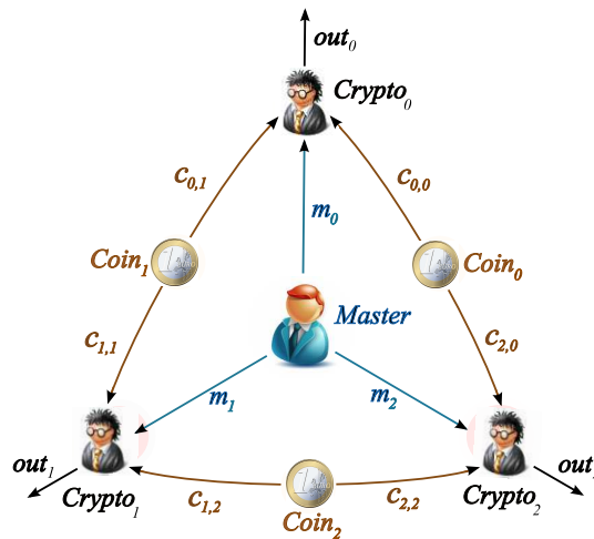
Figure 1: Chaum's system for the Dining Cryptographers ([13])
