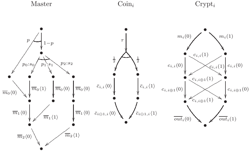
Figure 3: Dining Cryptographers Automata
