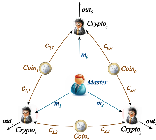
Figure 1: Chaum's system for the Dining Cryptographers ([13])
