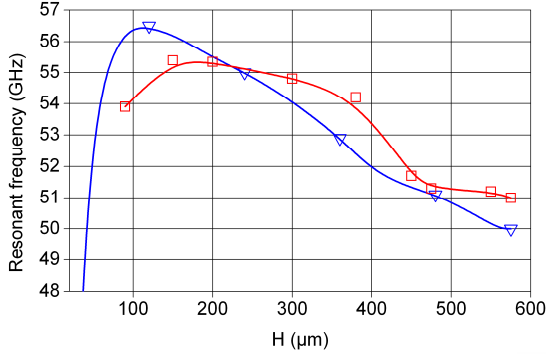
Fig. 6. Resonant frequency of the antenna as a function of H . \blacktriangledown HFSS simulations \blacksquare Experimental data.
