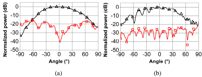
Fig.10. Measured radiation patterns of the inflated antenna (around H=575 \mu\text{m} ) at 50 GHz. (a) H-plane, (b) E-plane. \blacktriangle : Co-polarization component. \blacksquare : Cross-polarization component.
