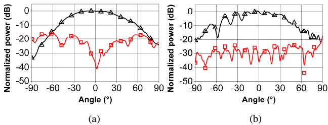
Fig.10. Measured radiation patterns of the inflated antenna (around H=575 \mu\text{m} ) at 50 GHz. (a) H-plane, (b) E-plane. \blacktriangle : Co-polarization component. \square : Cross-polarization component.
