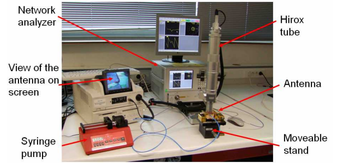
Fig. 4. Experimental setup.
