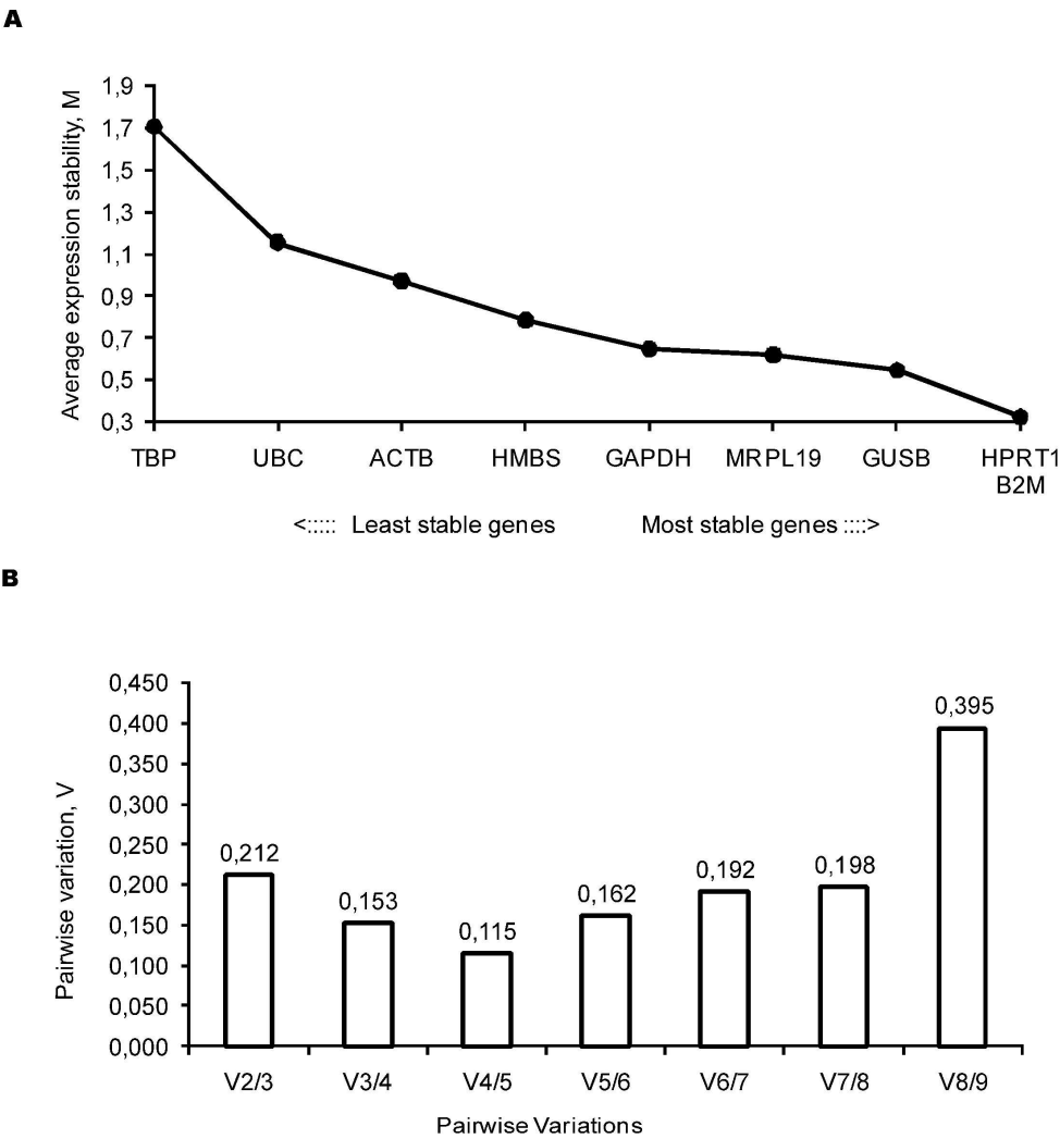
geNorm analysis of reference genes. Results are presented as an output file of the geNorm program. (A) Average expression stability (M) of reference genes during stepwise exclusion of the least stable gene. (B) Determination of the optimal number of reference genes for normalization. Every bar represents change in normalization accuracy when more reference genes are added stepwise according to the ranking. geNorm proposed cut-off value below which the inclusion of an additional reference gene is not required is 0.15.
