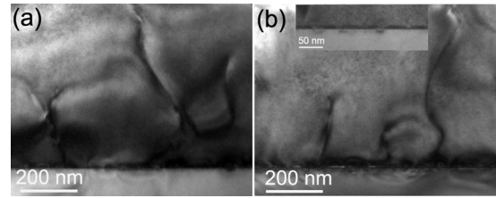
FIG. 2. Cross-sectional bright-field TEM images of sample B and D. The inset in (b) is a enlarge view of the interface showing the morphology of AlSb buffer.
