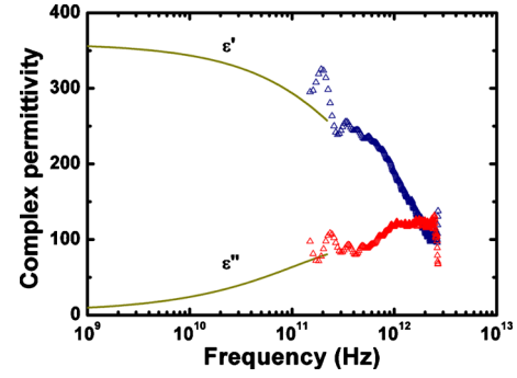
FIG. 4. (Color online) Complex permittivity as a function of frequency modeled by Cole-Cole function (solid lines) and measured by TDS (triangular points).
