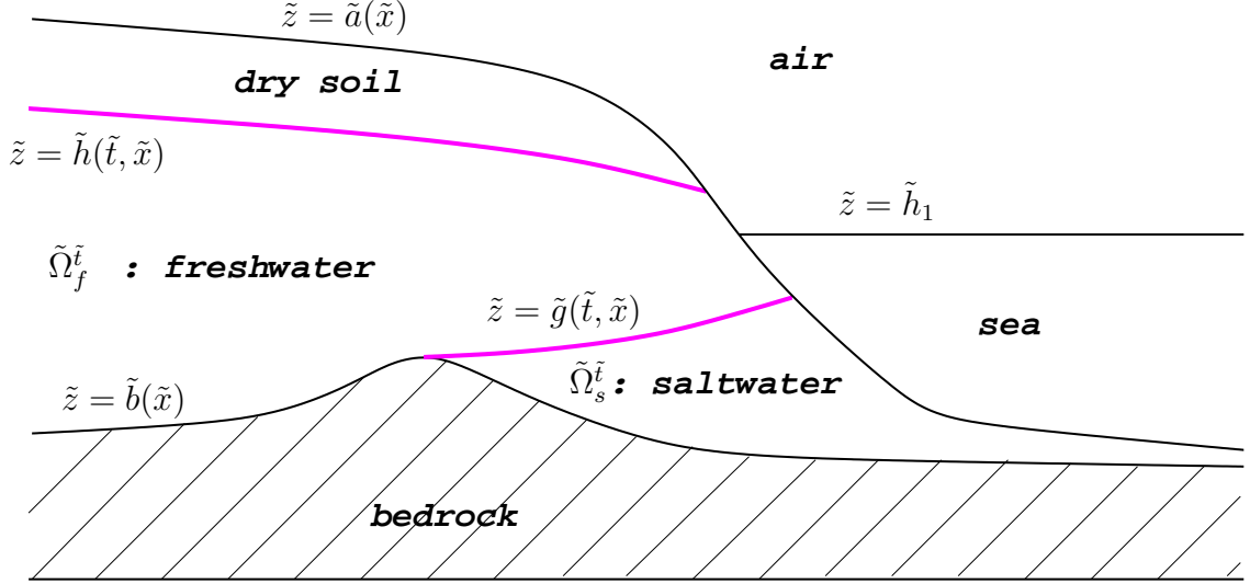
Figure 1: Unconfined aquifer
