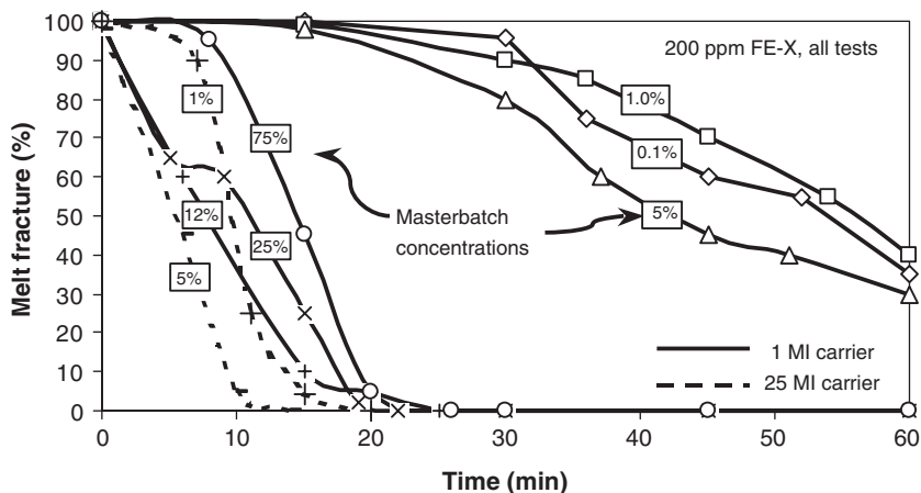
Figure 1. Melt fracture vs time, as a function of FE-X masterbatch concentration (Brabender® extruder with metering screw).
