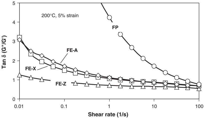
Figure 9. \tan \delta of fluoropolymers used in PPAs.
