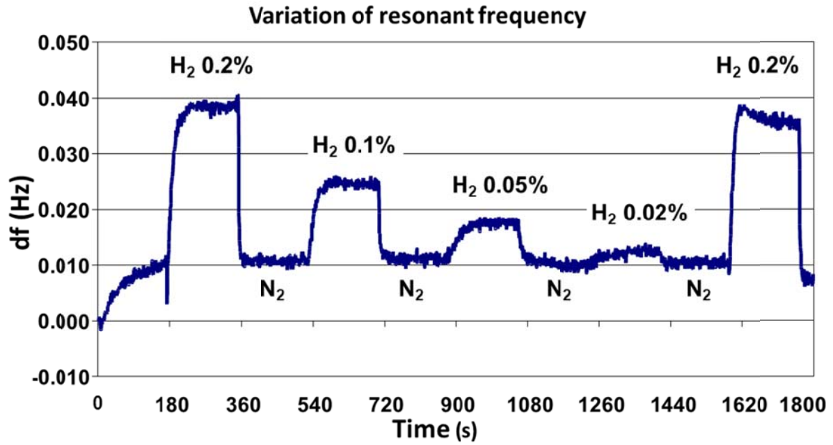
Fig. 4. Example of detection of small concentration of hydrogen in nitrogen with an uncoated 2000 \times 400 \times 15 \mu\text{m}^3 silicon cantilever
