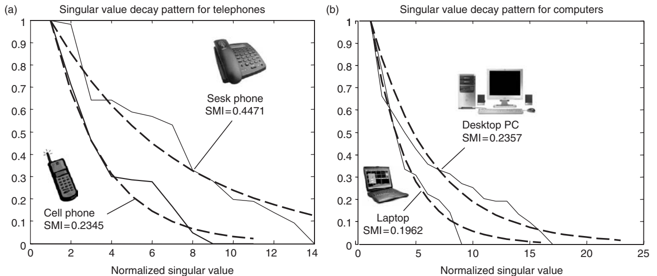
Figure 7. Singular value decay patterns for the pairs of telephones (left) and computers (right). A slower decay pattern (tendency towards the upper right) is indicative of a more modular architecture.
