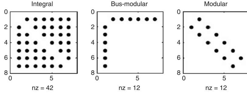
Figure 2. Sparsity pattern for idealized DSMs: (a) fully integral, (b) bus-modular, and (c) modular.
