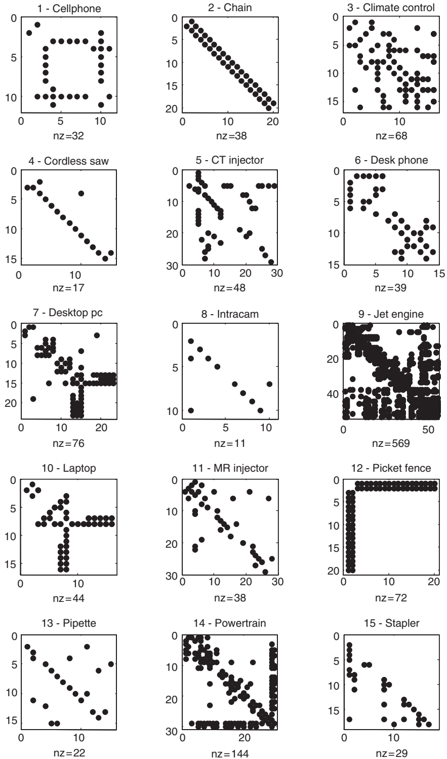
Figure 8. Sparsity patterns of binary DSM for 15 different systems and products: 1- cell phone, 2- chain, 3- climate control system [10], 4- cordless saw [33], 5- CT injector [32], 6- desk phone, 7- desktop PC, 8- intraoral camera [31], 9- jet engine [17], 10- laptop, 11- MR injector (unpublished sample), 12- picket fence, 13- electronic pipette [31], 14- powertrain [34], 15- stapler [35].
