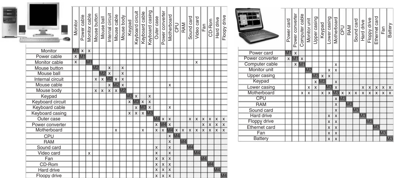
Figure 5. Component-to-component design structure matrix for two computers: desktop (left) and laptop (right).
