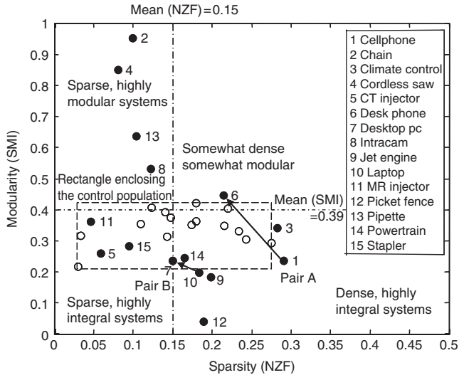
Figure 9. Modularity (SMI) versus sparsity (NZF) for 15 products and systems, plotted against a control group of 15 randomly generated systems (empty circles, enclosed by dashed box) with the same mean and standard deviation in terms of size ( N ) and sparsity (NZF).
