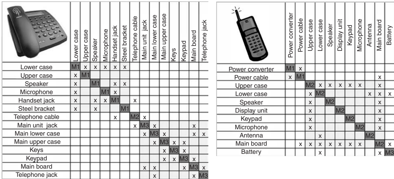
Figure 4. Component-to-component design structure matrix for two telephones: desk phone (left), cellular phone (right), the cellular phone is subject to volume (packaging) and lightweighting constraints.
