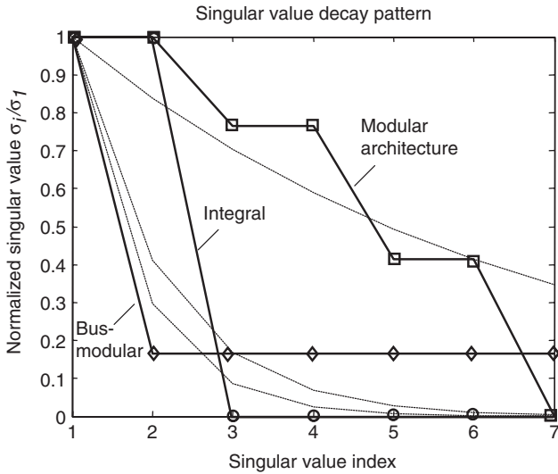
Figure 3. Singular values of the ‘integral’, ‘bus-modular,’ and ‘modular’ systems shown in Figure 1. Exponential approximation of decay patterns according to Equation (6) are shown by dashed lines.
