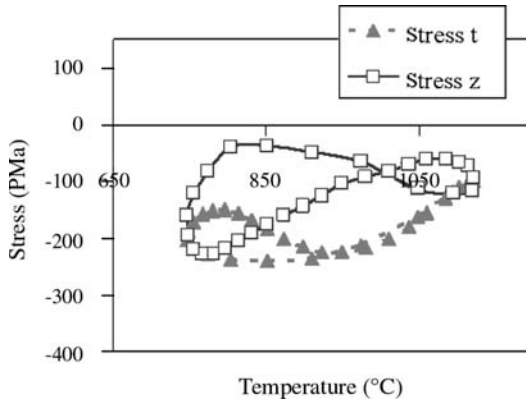
Figure 11. Thermomechanical cycle of external surface – with coating (longitudinal and
