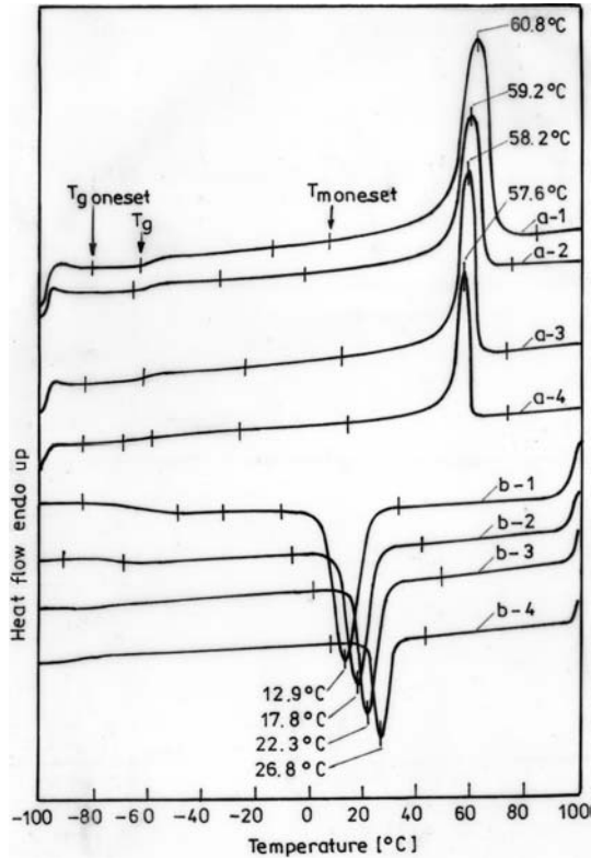
Figure 1. DSC diagrams for PCL: (a) heating from -100 to 100^\circ\text{C} and (b) cooling from 100 to -100^\circ\text{C} : (1) 36^\circ\text{C}/\text{min} ; (2) 25^\circ\text{C}/\text{min} ; (3) 16^\circ\text{C}/\text{min} ; (4) 9^\circ\text{C}/\text{min} .
