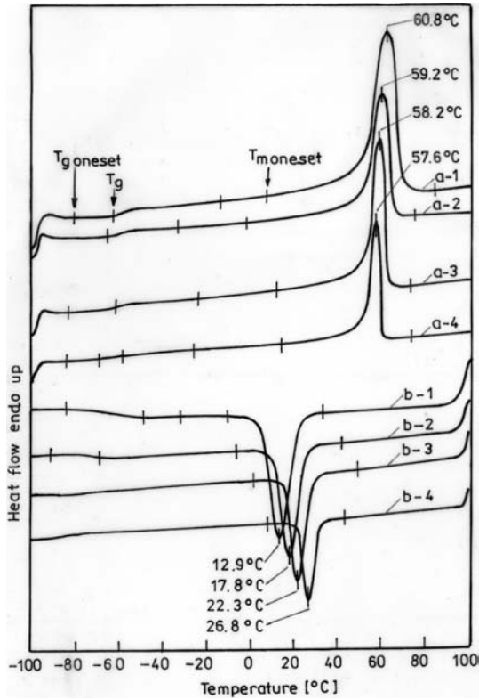
Figure 1. DSC diagrams for PCL: (a) heating from -100 to 100^\circ\text{C} and (b) cooling from 100 to -100^\circ\text{C} : (1) 36^\circ\text{C}/\text{min} ; (2) 25^\circ\text{C}/\text{min} ; (3) 16^\circ\text{C}/\text{min} ; (4) 9^\circ\text{C}/\text{min} .
