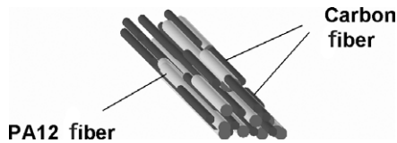
Figure 1. CF–PA12 hybrid yarn.
