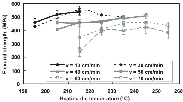
Figure 10. Flexural strength as a function of heating die temperature.
