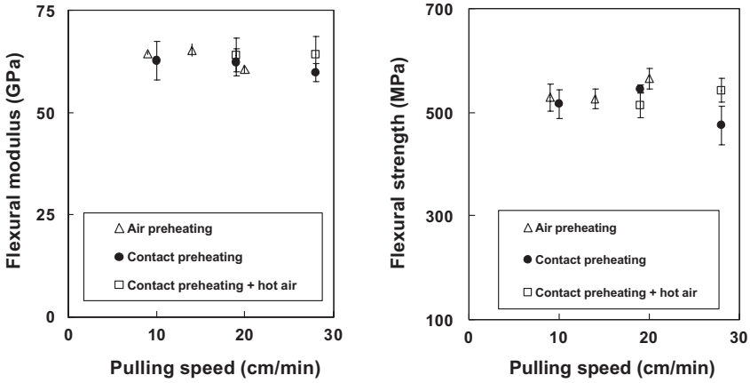
Figure 5. Flexural strength and flexural modulus vs pulling speed using different preheating methods.
