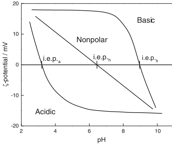
Figure 1. Schematic picture of \zeta = f(\text{pH}) for Brønsted acidic and alkaline surface functional groups and for complete hydrophobic (i.e., nonpolar) surfaces.
