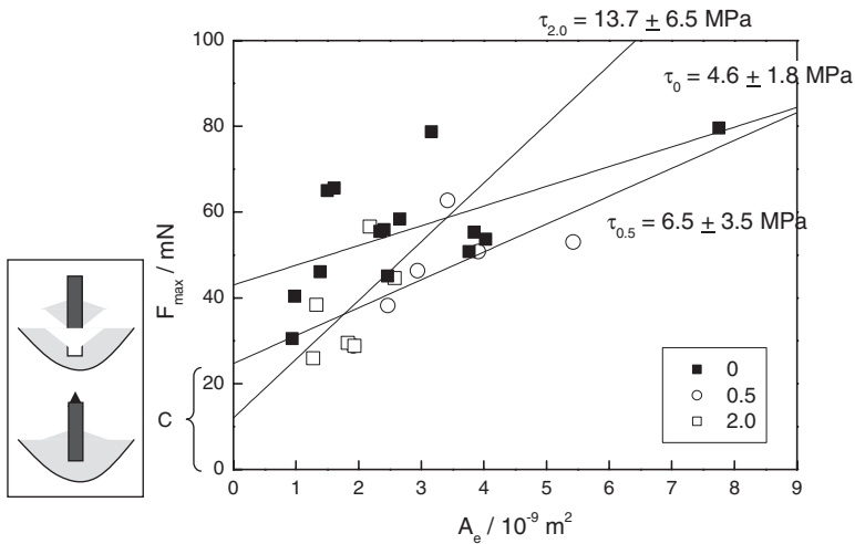
Figure 8. The maximum pull-out force F_{max} of the unmodified, original fiber (0) and the PS-grafted fibers (0.5 and 2.0) as function of the embedded fiber area. The resulting intercept C is due to the formation of a collar (fractured wetting cone) still attached to the fiber (see also Figures 9 and 10 (c), (d)) after being pulled out of the matrix, which is diagrammatically shown in the insert.
