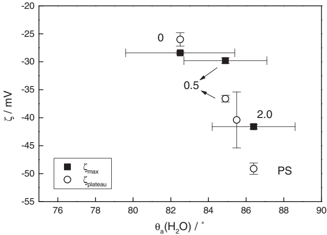
Figure 5. \zeta -Potential ( \zeta_{plateau} and \zeta_{max} ) as function of advancing water contact angles \theta_a(H_2O) .
