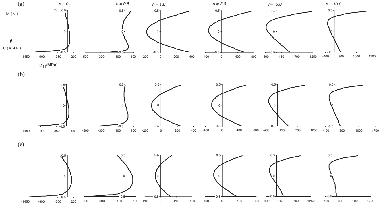
Figure 7. The effect of the compositional gradient exponent n on the through-thickness variation of the longitudinal stress \sigma_{11} in Ni- \text{Al}_2\text{O}_3 functionally graded plates subjected to: (a) uniform; (b) linear; and (c) parabolic temperature fields (stresses in MPa).
