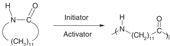
Figure 1. Schematic of anionic polymerization of PA12.
