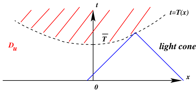
Fig. 1: The maximal influence domain of the solution
