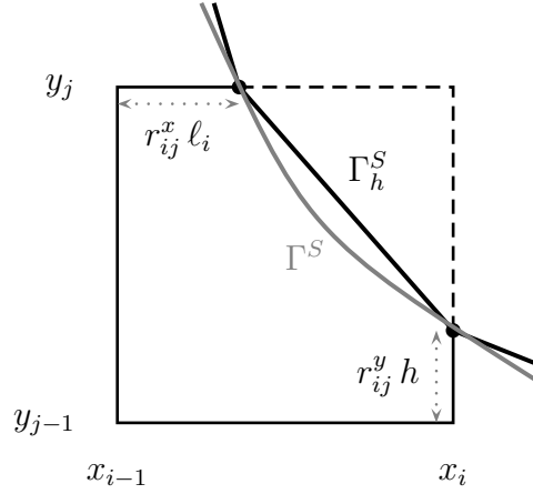
Figure 2: The discrete representation \Gamma_h^S of the immersed boundary \Gamma^S .
