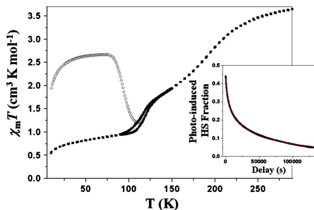
FIG. 2. (Color online) Temperature dependence of the \chi_M T product. \chi_M T follows the law (\chi_M T) \sim \frac{1}{8} g^2 [S(S+1)] where \chi_M is the molar magnetic susceptibility, T the temperature, g the Landé factor ( g \approx 2 ), and S the molecular spin state. The closed circles show a thermal cycle (295 K–2 K–295 K) recorded in the dark, while the open circle symbols show the evolution of \chi_M T in the dark when heating the sample from 10 to 130 K following light irradiation (647 nm) at 10 K under irradiation. (Insert) Relaxation of the metastable HS fraction observed at 90 K, i.e., slightly below T(\text{LIESST}) . The experimental curve (black) is well fitted by a stretched exponential law, thus introducing a Gaussian width of the activation energy of 100 \text{ cm}^{-1} .
