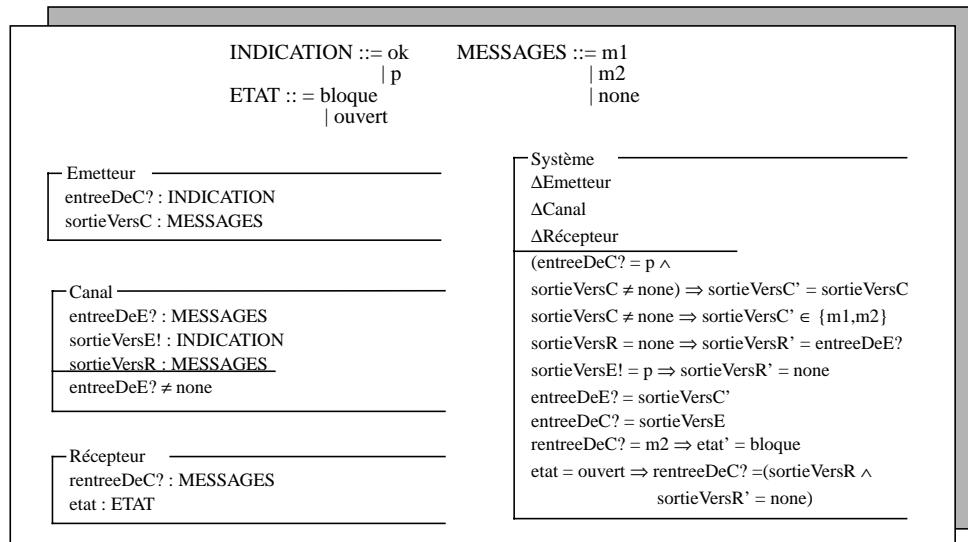
Figure 5. Spécification in Z of the Transmission.
