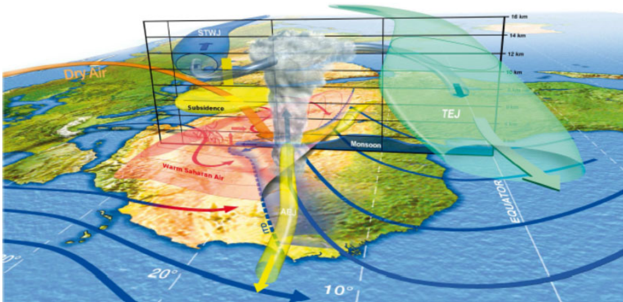
Figure 1. Three-dimensional schematic view of the WAM. ITD, inter-tropical discontinuity; TEJ, tropical easterly jet; STWJ, subtropical westerly jet; AEJ, African easterly jet. The oscillation of the AEJ yellow tube figures an African easterly wave [from Lafore et al. (2010)].
