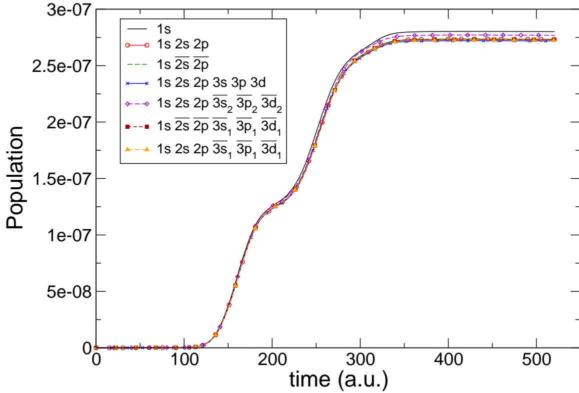
Figure 4. Population of the external region for the length gauge using a pulse frequency of \omega = 0.24 a.u. for 6 cycles at a peak intensity of 2 \times 10^{13} W cm ^{-2} . Details on the basis sets used are given in the caption to figure 2.
