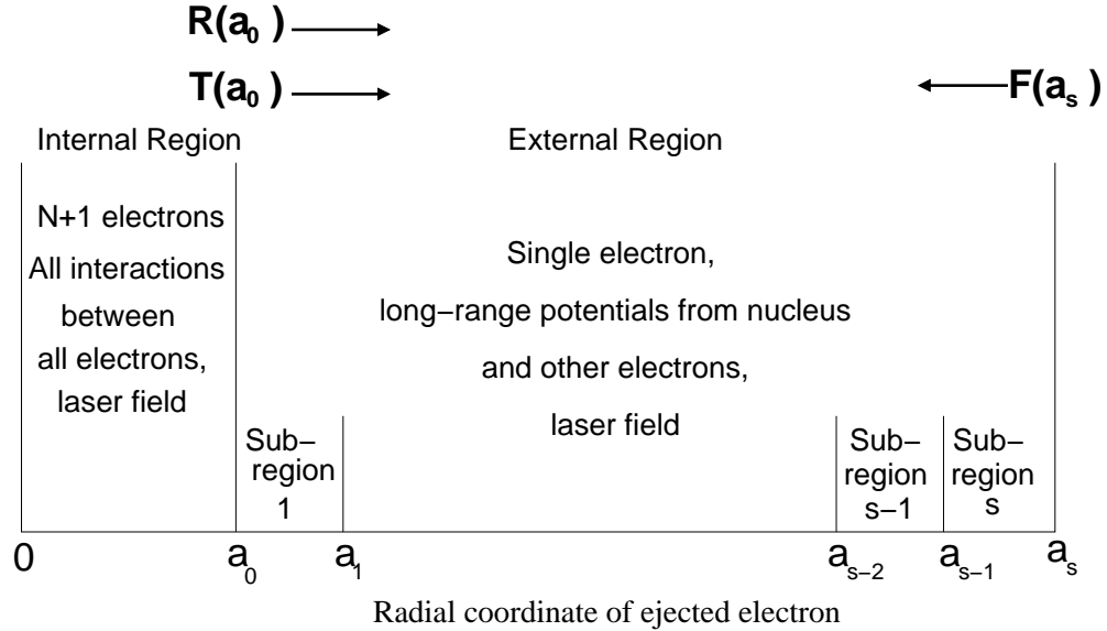
Figure 1. Partition scheme for the configuration space
