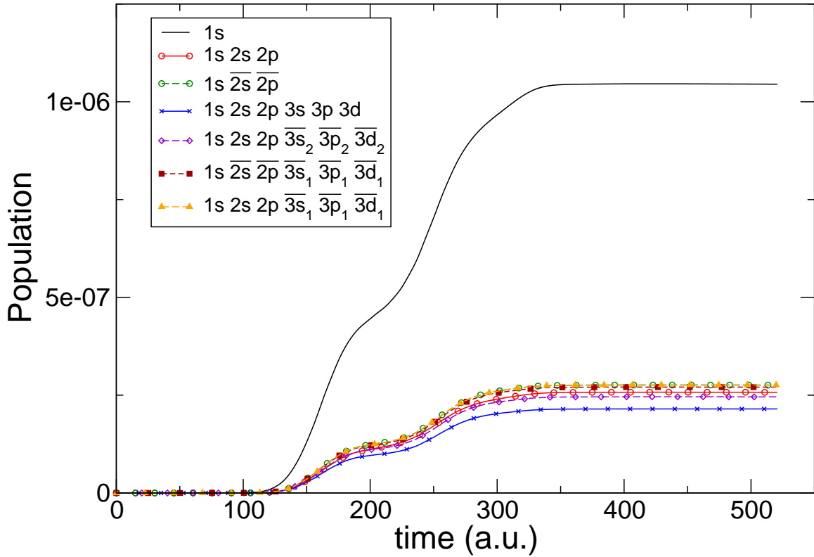
Figure 5. Population of the external region for the velocity gauge using a pulse frequency of \omega = 0.24 a.u. for 6 cycles at a peak intensity of 2 \times 10^{13} W cm ^{-2} . Details on the basis sets used are given in the caption to figure 2.
