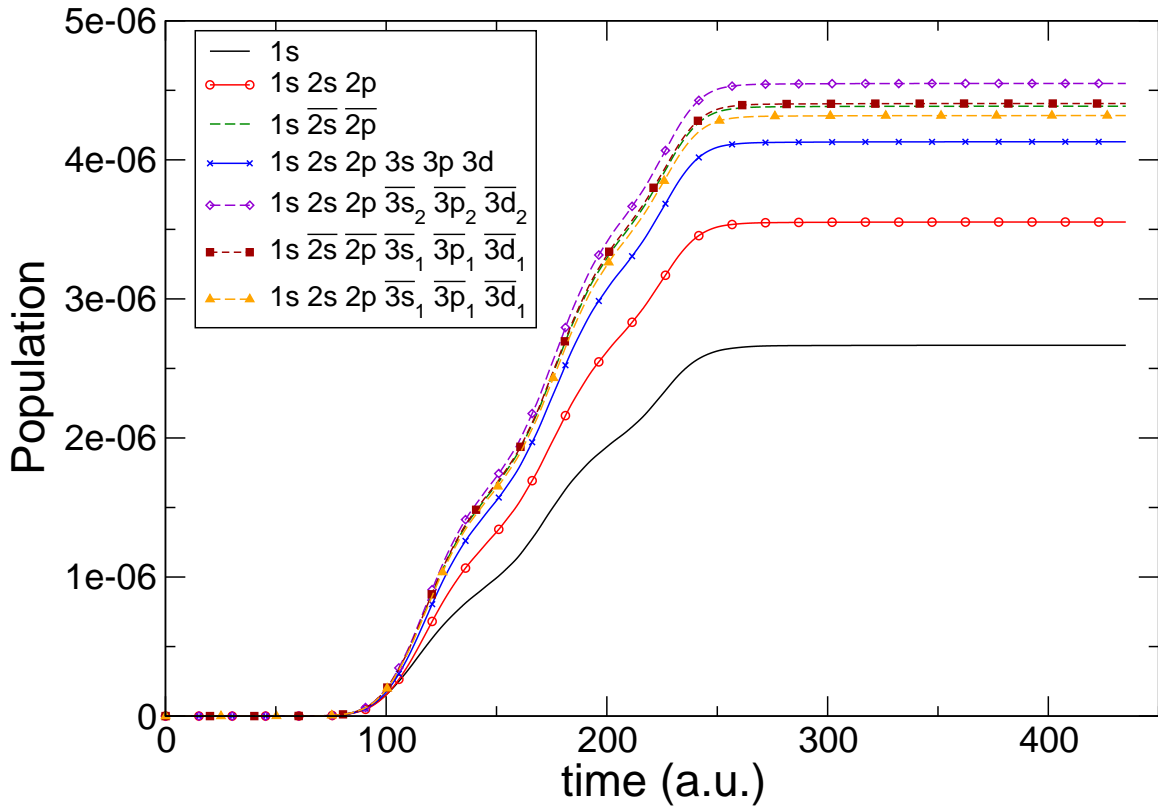
Figure 3. Population of the external region for various basis sets using the velocity gauge with a laser frequency of \omega = 0.33 a.u. for 6 cycles at a peak intensity of 2 \times 10^{13} W cm ^{-2} . Details on the basis sets used are given in the caption to figure 2.
