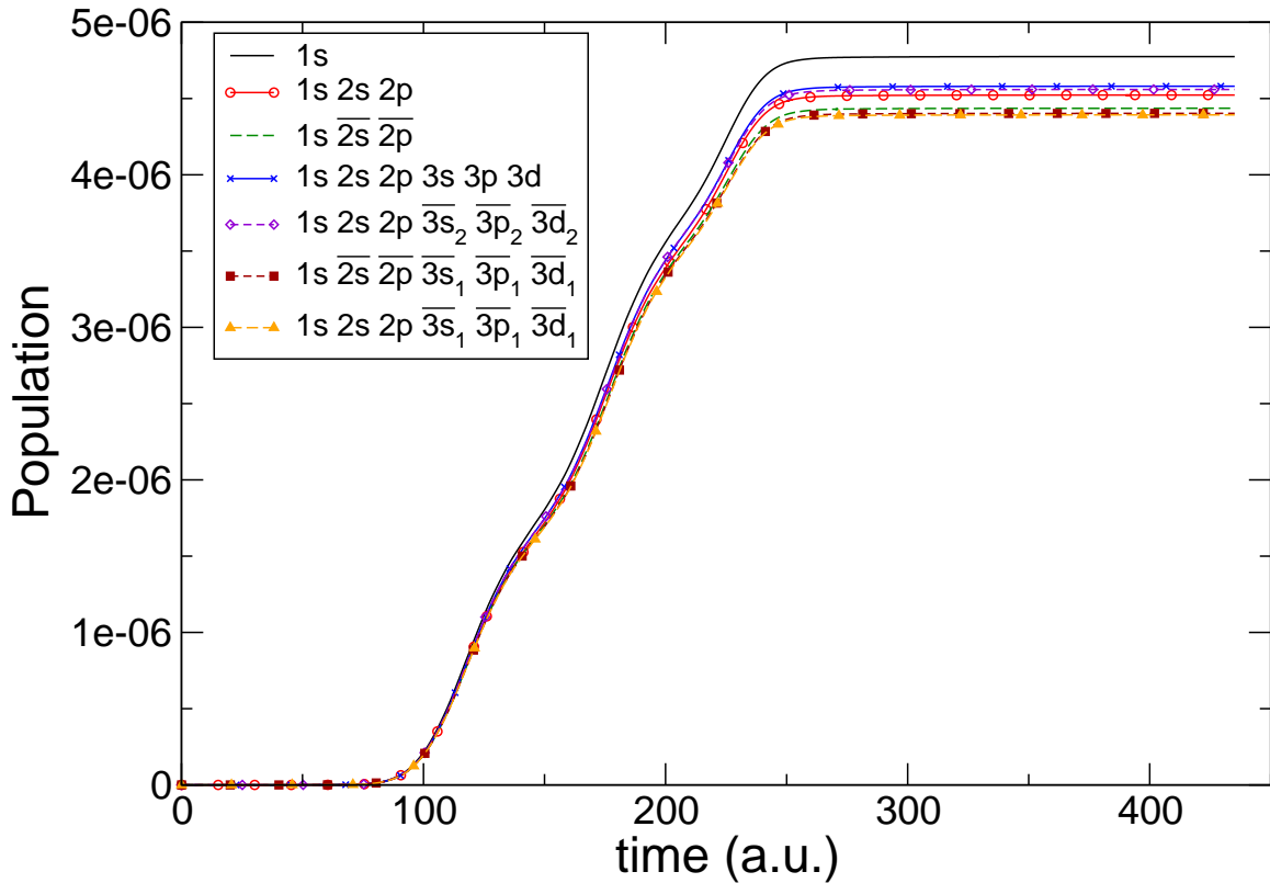
Figure 2. Population of the external region ( r > 30 a.u.) for various basis sets using the length gauge and a pulse frequency of \omega = 0.33 a.u. with 6 cycles at a peak intensity of 2 \times 10^{13} \text{W cm}^{-2} . The basis sets used are defined in terms of the states of \text{He}^+ included. Shown are basis sets including the real (solid lines) \text{He}^+ orbitals 1s (black), 1s 2s 2p (red, circles) and 1s 2s 2p 3s 3p 3d (blue, crosses) along with those involving pseudo-states of \text{He}^+ (dashed lines) 1s \overline{2s} \overline{2p} (dark green), 1s 2s 2p \overline{3s_1} \overline{3p_1} \overline{3d_1} (orange, solid triangles), 1s 2s 2p \overline{3s_2} \overline{3p_2} \overline{3d_2} (purple, diamonds), 1s \overline{2s} \overline{2p} \overline{3s_1} \overline{3p_1} \overline{3d_1} (dark red, solid squares). Here a subscript on an orbital indicates the exponential behaviour of the orbital.
