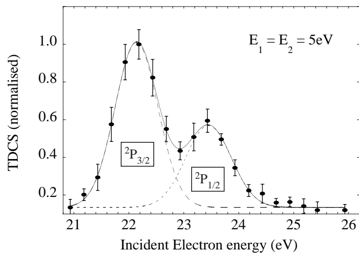
FIG 7. Energy loss spectrum for the ionization of xenon in the perpendicular plane, with incident energy 10eV above the ionization potential, showing the resolution of the ^2P_{3/2}, ^2P_{1/2} ionic ground states. The data are fitted to two Gaussians, showing that contamination from each ionic state is <10% when the spectrometer is set to each peak in the cross section.
