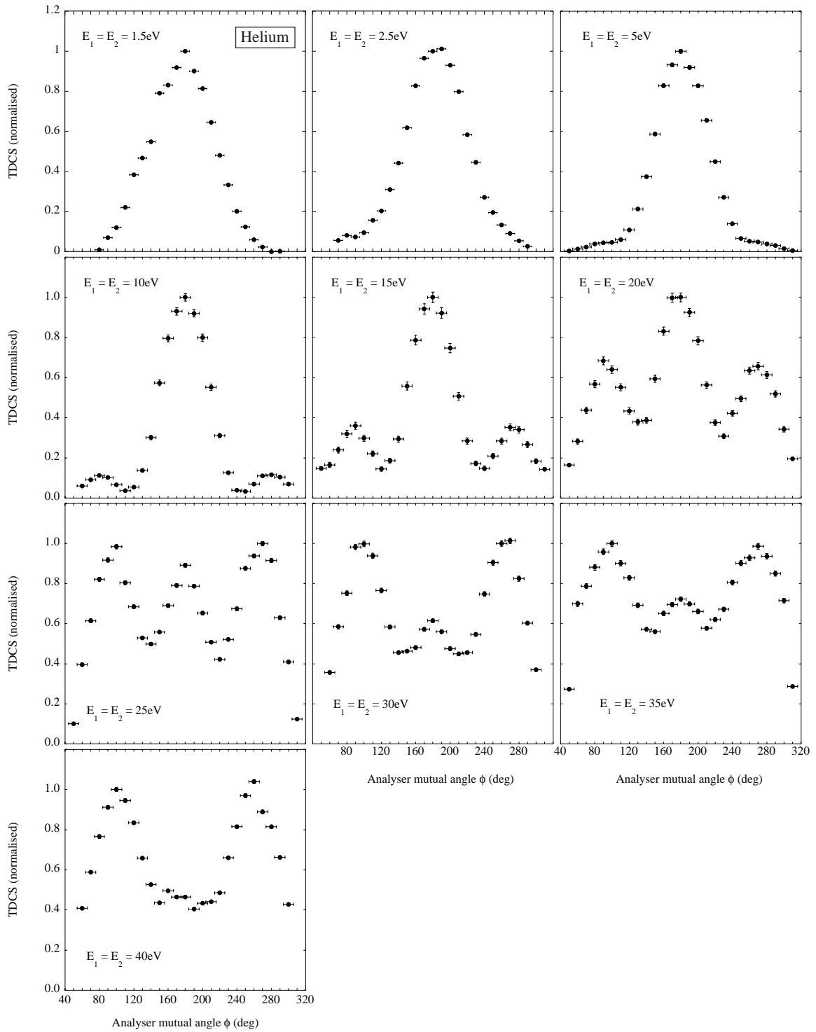
FIG 3. Experimental results for the ionization of helium in the perpendicular plane, with incident energies ranging from 3eV to 80eV above the ionization potential for this target. For details, see text.
