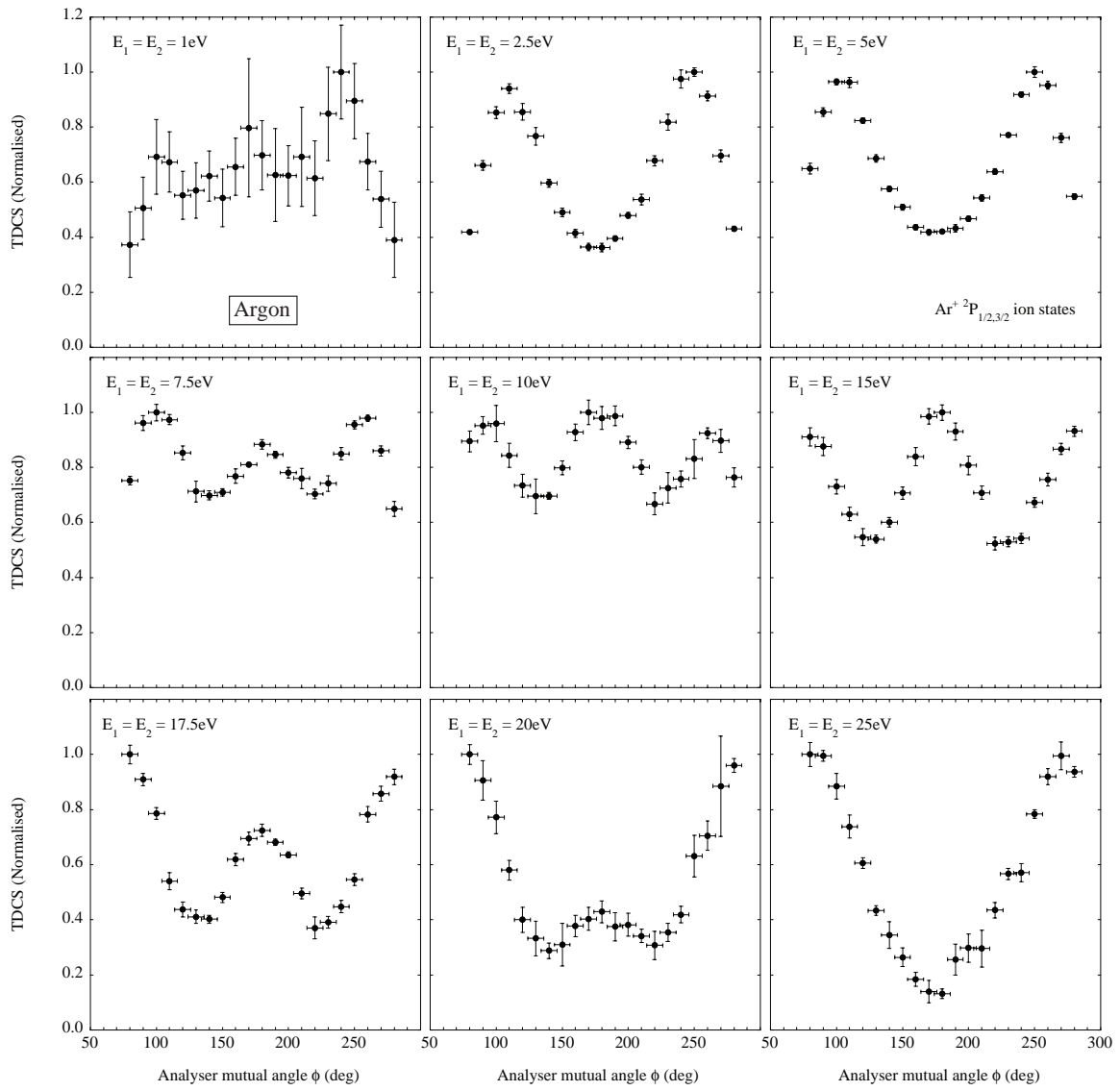
FIG 5. Experimental results for the ionization of argon in the perpendicular plane, with incident energies ranging from 2eV to 50eV above the ionization potential for this target.
