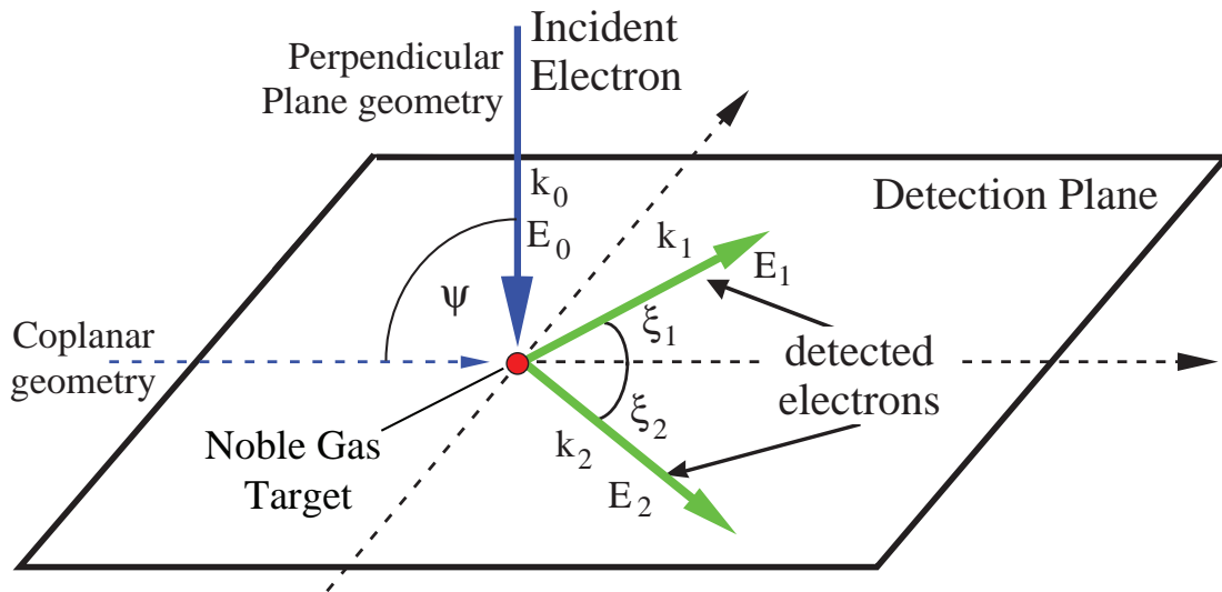
FIG 1. The experimental geometry adopted in Manchester. The incident electron can move from the coplanar geometry ( \psi = 0^\circ ) to the perpendicular plane ( \psi = 90^\circ ), the outgoing electrons are measured in the detection plane. For the data presented here, the perpendicular plane was chosen, so only the mutual angle \phi = \xi_1 + \xi_2 is relevant.
