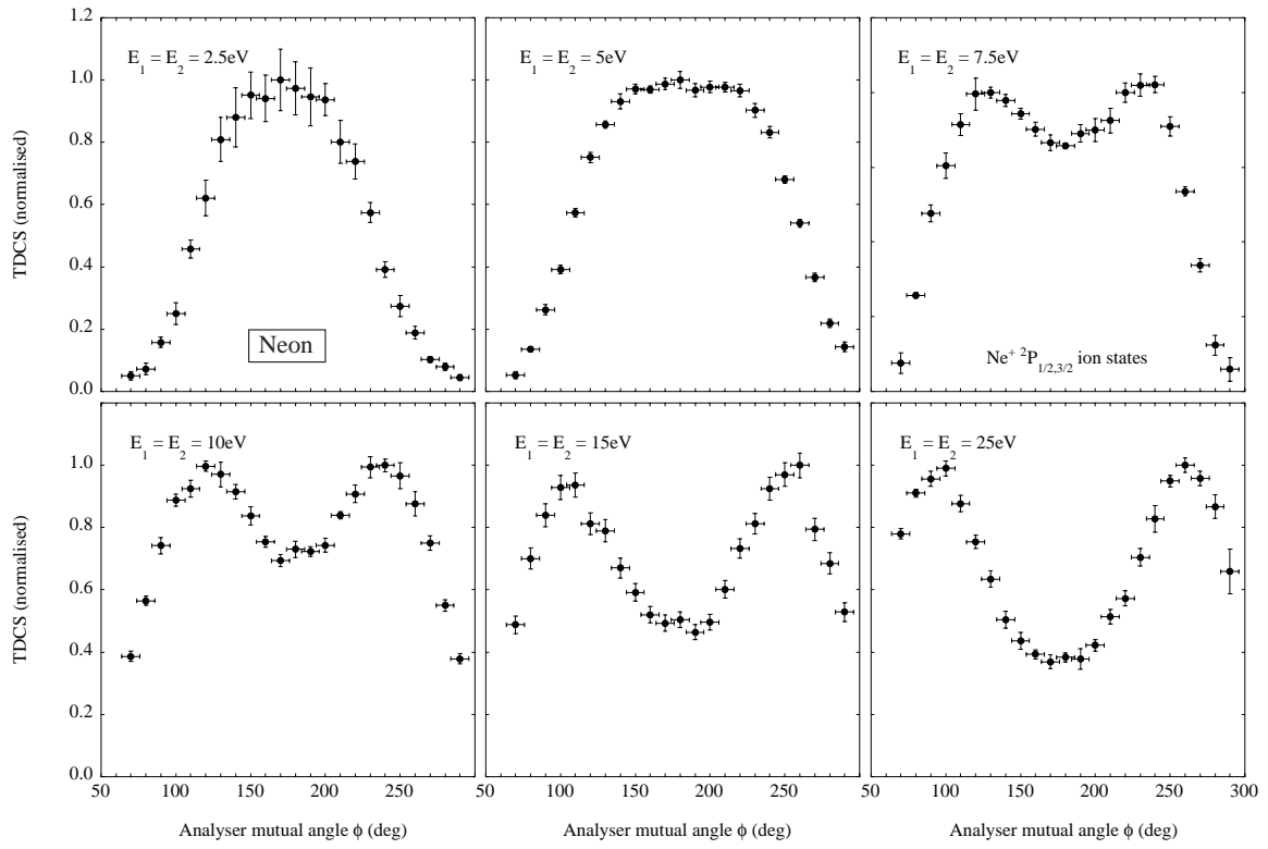
FIG 4. Experimental results for the ionization of neon in the perpendicular plane, with incident energies ranging from 5eV to 50eV above the ionization potential for this target. For details, see text.
