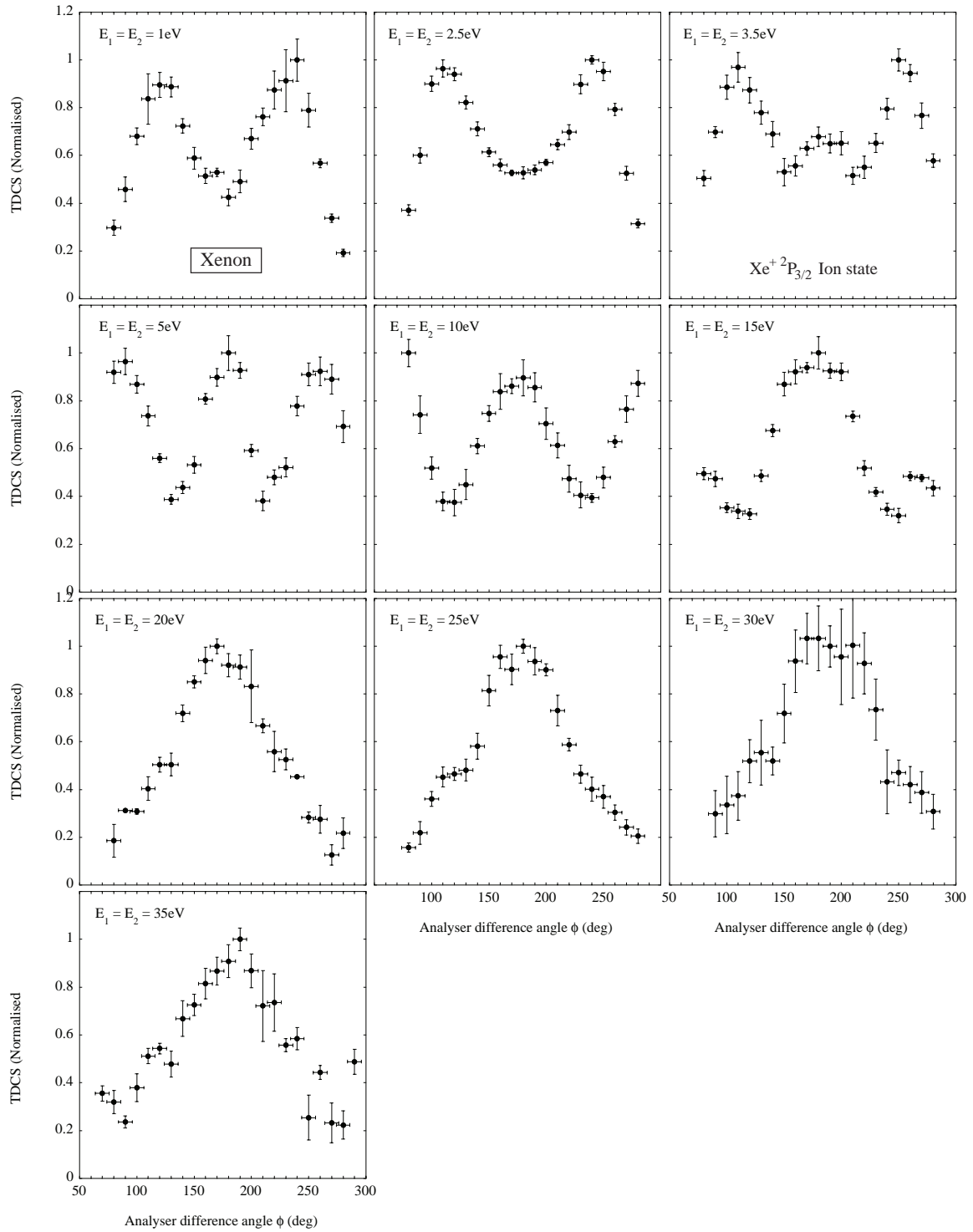
FIG 8. Experimental results for the ionization of xenon taken in the perpendicular plane, with incident energies ranging from 2eV to 70eV above the ionization potential for this target. For Energies up to 30eV above the IP the results represent those of the resolved 2 P 3/2 ionic ground state. At higher energies the data measured has contributions from both ion states, but is expected to be dominated by the 2 P 3/2 state.
