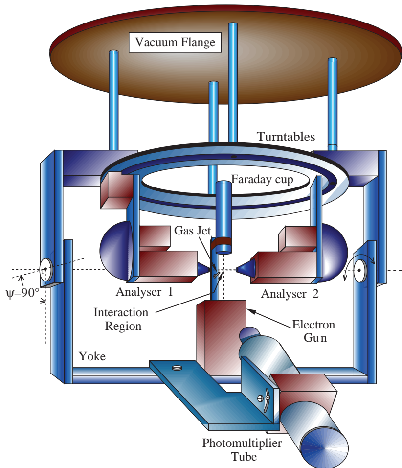
FIG 2. The (e,2e) spectrometer used in these experiments, configured in the perpendicular plane. For details, see text.
