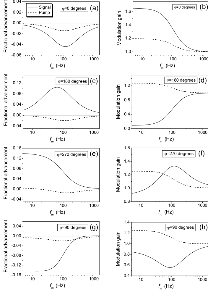
Figure 7. Simulated fractional advancement of the signal (solid line) and pump (dashed line) as a function of the modulation frequency for different relative phases between the signal and pump modulated beams: \varphi = 0 (a) \varphi = \pi (c), \varphi = 3\pi/2 (e), and \varphi = \pi/2 (g). Simulated modulation gain for the signal [(P_{sm}/P_{s0})_{out}/(P_{sm}/P_{s0})_{in}] (solid line) and pump (dashed line) as a function of the modulation frequency for \varphi = 0 (b) \varphi = \pi (d), \varphi = 3\pi/2 (f), and \varphi = \pi/2 (h). P_{s0} = 0.9 with P_{sm} = 0.4P_{s0} , and P_{p0} = 4.4 with P_{pm} = 0.7P_{p0} .
