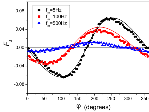
Figure 3. Fractional advancement of the signal as a function of the relative phase between the signal and pump modulated beams for three different modulation frequencies. Experiments (symbols) and simulations (lines). Signal power = 0.14 mW ( P_{s0} = 0.24 ). Pump power = 10 mW ( P_{p0} = 4.3 ). Modulation depths P_{sm}/P_{s0} = P_{pm}/P_{p0} \simeq 0.5 .
