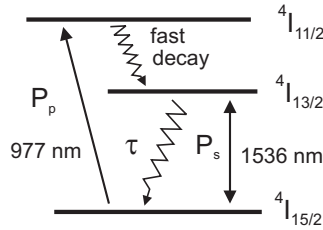
Figure 1. Three-level system for \text{Er}^{3+} ions. Wavelengths for the signal and pump beams.
