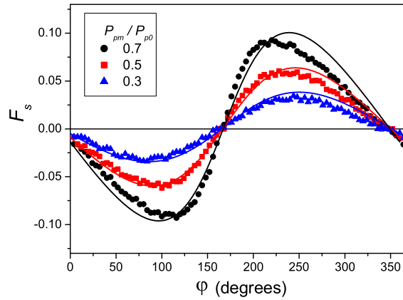
Figure 5. Fractional advancement of the signal as a function of the relative phase between the signal and pump modulated beams for three different pump modulation depths. Experiments (symbols) and simulations (lines). f_m = 20 Hz. The rest of parameters are the same than the ones used in figure 3.
