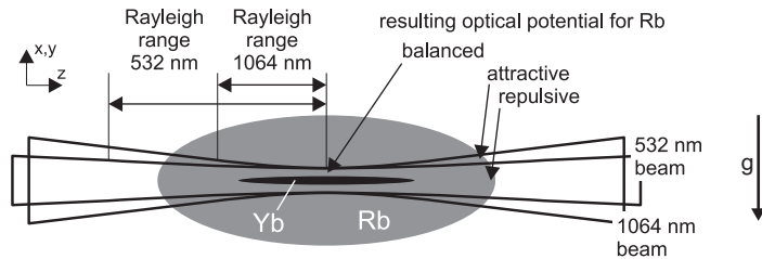
Figure 1. Scheme of the combined trap with the spatial configuration of the atomic clouds and the BIODT laser beams (not to scale).
