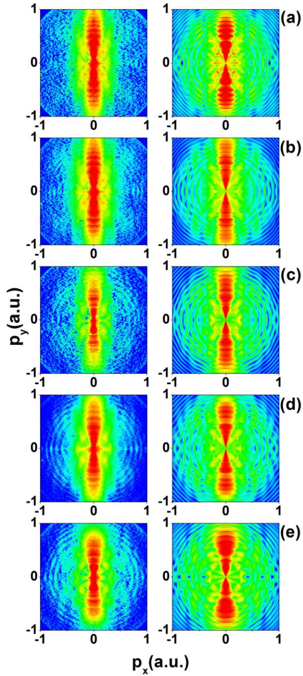
Figure 1. (Colour online) Experimental (left column) and calculated (right column) momentum maps for ionization of Ar at various wavelengths and intensities (from top to bottom): (a) 800 nm, A_{\max}=0.85 a. u., 0.82 \times 10^{14} W/cm 2 ; (b) 750 nm, A_{\max}=0.98 a. u., 1.25 \times 10^{14} W/cm 2 ; (c) 700 nm, A_{\max}=0.88 a. u., 1.15 \times 10^{14} W/cm 2 ; (d) 650 nm, A_{\max}=0.93 a. u., 1.48 \times 10^{14} W/cm 2 ; (e) 600 nm, A_{\max}=0.78 a. u., 1.23 \times 10^{14} W/cm 2 . The logarithmic false-colour scale covers three orders of magnitude.
