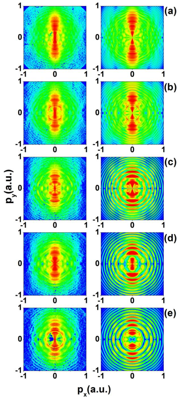
Figure 5. (Colour online) Experimental (left column) and calculated (right column) momentum maps for ionization of Xe at various wavelengths and intensities (from top to bottom): (a) 800 nm, A_{\max}=0.77 a.u., 6.7\times 10^{13} W/cm 2 ; (b) 740 nm, A_{\max}=0.7 a.u., 6.4\times 10^{13} W/cm 2 ; (c) 700 nm, A_{\max}=0.55 a.u., 4.5\times 10^{13} W/cm 2 ; (d) 650 nm, A_{\max}=0.52 a.u., 4.6\times 10^{13} W/cm 2 ; (e) 600 nm, A_{\max}=0.53 a. u., 5.7\times 10^{13} W/cm 2 . The logarithmic false-colour scale covers four orders of magnitude.
