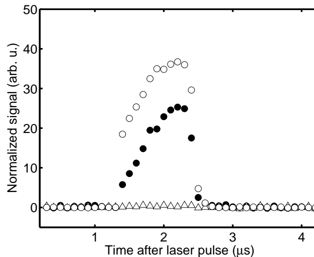
Figure 6. Neutral detector counts as a function of time, measured for silicon with cooler off ( \circ ), cooler on ( \bullet ), and cooler on plus the depletion laser ( \triangle ). The data have been normalized with respect to the ion current. Each curve corresponds to the integrated signal from 10 000 laser pulses. This data was recorded with 600 mW depletion laser power (measured after the magnet), a He pressure of 3 \times 10^{-2} and 10 V on the DC electrodes in the cooler.
