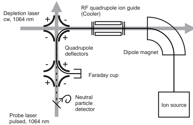
Figure 2. The experimental set-up showing the depletion laser passing through the ion cooler and the probe laser applied in the probe region between the two quadrupoles. Both laser powers are measured external to the vacuum system.
