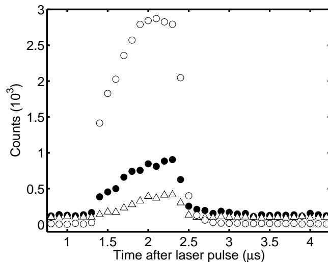
Figure 4. Neutral detector counts as a function of time, measured for silicon with cooler off ( \circ ), cooler on ( \bullet ), and cooler on plus the depletion laser interacting with the ions inside the cooler ( \triangle ). This data was recorded with 50 mW depletion laser power (measured after the magnet), a He pressure of 2 \times 10^{-2} and 14 V on the DC electrodes in the cooler.
