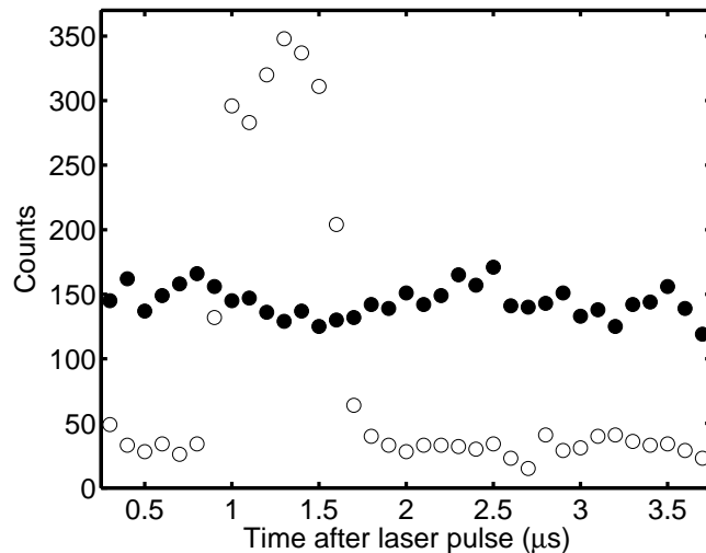
Figure 3. Neutral detector counts as a function of time, measured for C^- beams without ( \circ ) and with ( \bullet ) the cooler in operation. Each curve corresponds to the sum of counts generated by 10 000 probe laser pulses.
