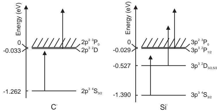
Figure 1. Energy levels of C and Si. The arrows indicate the photon energy (1.165 eV) of the fundamental radiation from a Nd:YAG laser that was used in the experiment. The photon energy is less than the binding energy of the ground state in both Si - and C - .
