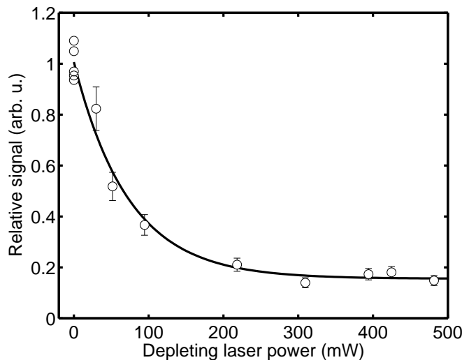
Figure 5. Relative population in the ^2\text{D} excited state of \text{Si}^- as a function of the depletion laser power, obtained with a He pressure of 2 \times 10^{-2} and 14 V on the DC electrodes in the cooler.
