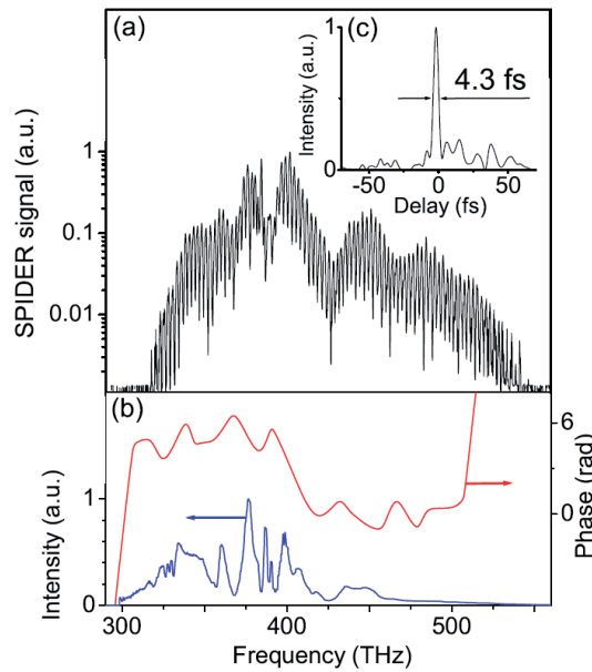
Figure 30. Taken from [156]: High Dynamic Range SPIDER measurement of a 4.3 fs pulse out of a fibre compressor. (a) SPIDER interferogram, (b) reconstructed spectral phase and amplitude, (c) temporal intensity profile.
