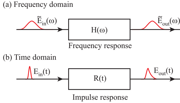
Figure 4. Pulse shaping by linear filtering. (a) Frequency domain. (b) Time domain.
