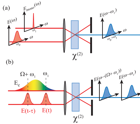
Figure 28. Spectral shearing by upconversion: (a) the upconversion between E(\omega) a quasi-monochromatic pulse E_{mono}(\omega) centered around \omega_1 generates a spectrally shifted replica E(\omega - \omega_1) ; (b) the upconversion between two delayed replicas E(t) and E(t - \tau) and a chirped pulse E_c(t) leads to two delayed and spectrally shifted replicas.
