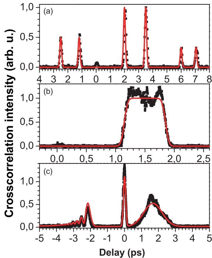
Figure 10. Three experimental waveforms (black dots) are presented: (a) three equal amplitude pulses pairs with relative intensity 1/2:1:1/3, (b) a square pulse of 700 fs, and (c) three pulses with cubic, flat and quadratic phase. The solid red line is the analytical desired wave form intensity.
