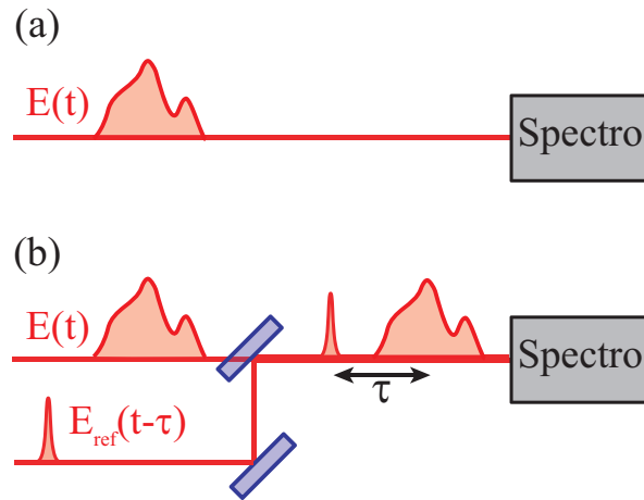
Figure 19. Spectral interferometry: The test pulse E(t) is sent into a spectrometer either (a) alone to measure spectral amplitude or (b) together with a delayed reference pulse E_{ref}(t - \tau) to retrieve the spectral phase.
