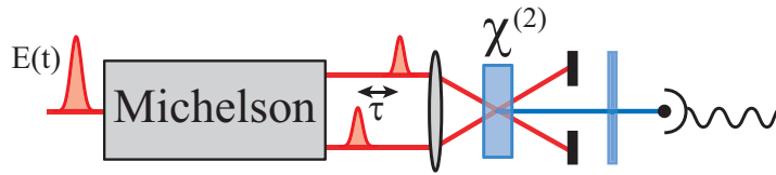
Figure 21. Intensimetric autocorrelator: the two delayed replicas are focused in the crystal with an angle and only the cross-term of the second harmonic is recorded.
