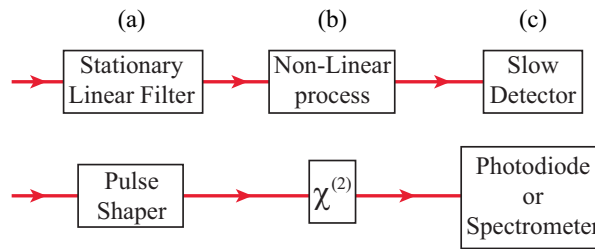
Figure 32. Generic set-up for complete characterization: (a) a pulse shaper serves as a generic versatile linear filter, followed by (b) a non-linear process which output is monitored by (c) a slow detector.
