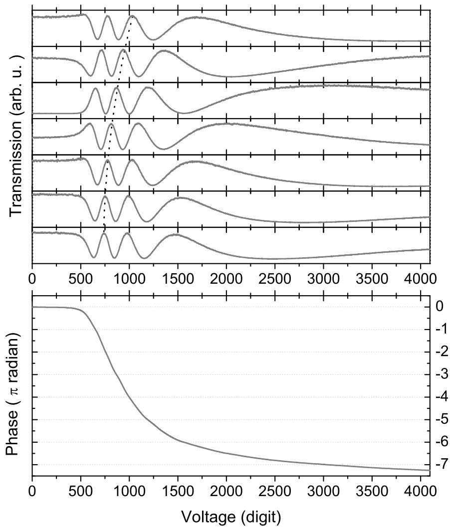
Figure 8. Phase-voltage calibration at 795 nm of a CRI128 LC-SLM: Top curves: transmitted intensity as a function of the applied voltage, for several orientation of the waveplate; the position of the extrema depends on the extra phase added by the waveplate (dashed line is a guide to the eye). Bottom curve: Reconstructed phase as a function of the voltage.
