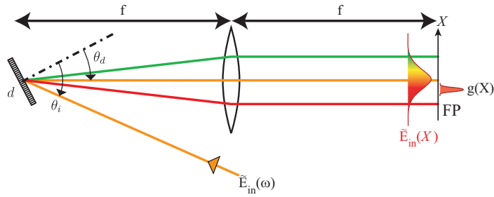
Figure 5. Half a 4f line : The Fourier plane is situated in the back focal plane of the lens. f is the focal length. X is the spatial coordinate in this plane. g(X) is the spatial extension of a given frequency component. \theta_i is the incident angle on the grating. d is the grating period. \theta_d the diffraction angle.
