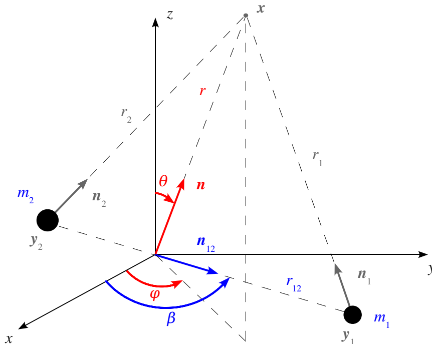
Figure 1. Two black holes of Schwarzschild masses m_{1,2} in a Cartesian coordinate system x^\mu = \{ct, x, y, z\} centered on the binary's center of mass, or the associated spherical coordinate system x^\alpha = \{ct, r, \theta, \varphi\} .
