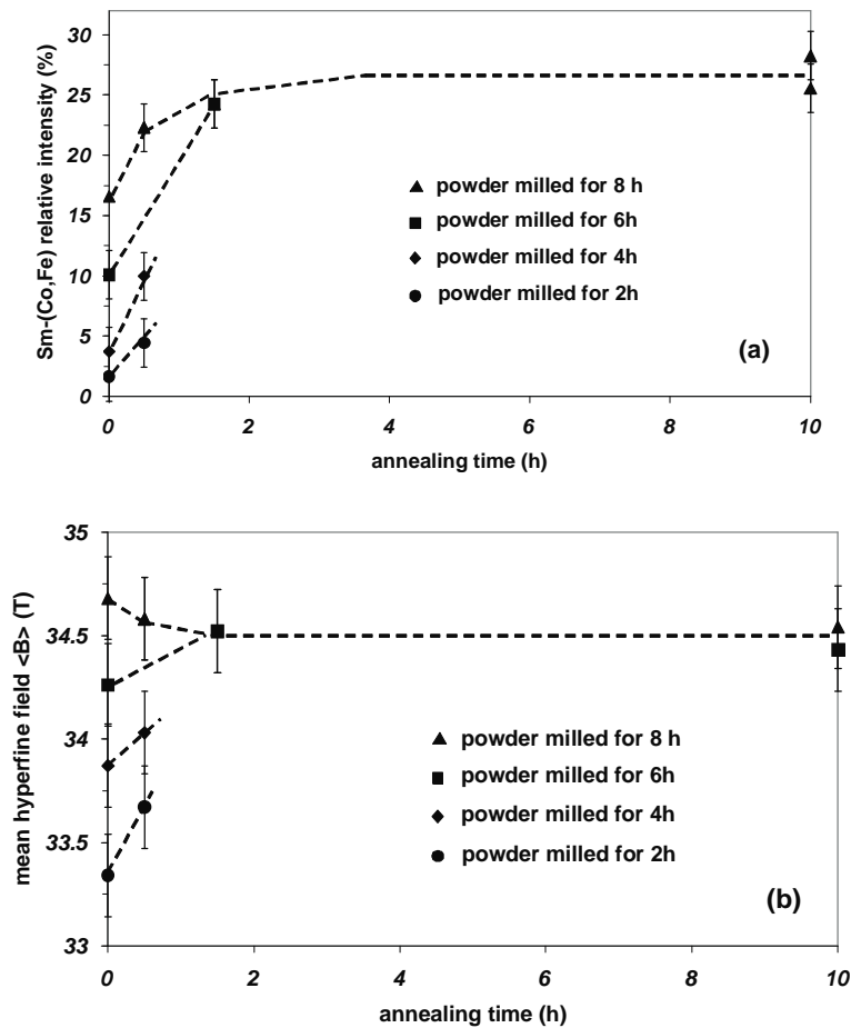
Figure 7. Evolution with the annealing time at 450°C of (a) the relative intensity of the Sm(Co,Fe) 5 contribution, and (b) the mean hyperfine field of the \alpha -Fe(Co) contribution. The lines are guides for the eye.
