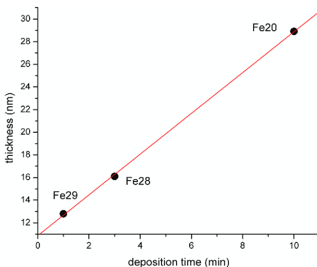
Figure 1. Grow rate of the Fe 3 O 4 films listed in table 1. The red line shows a linear fit of the samples thickness depending on different deposition times.
