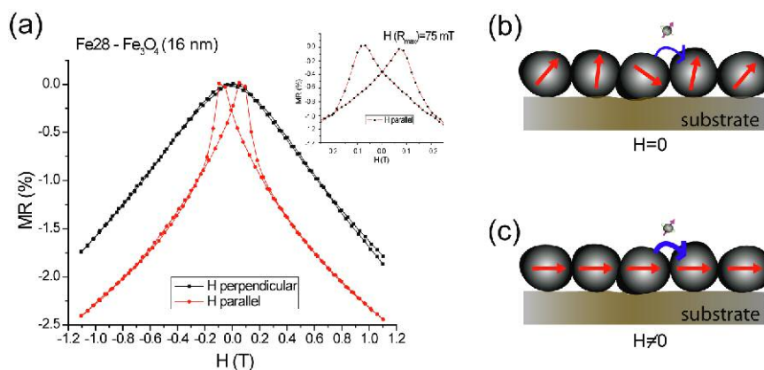
Figure 9. (a) MR measurements at RT of sample Fe28 for an applied field up to 1.1 T applied both parallel and perpendicular to the film plane; (b) without an applied magnetic field, the magnetizations of the grains are almost randomly oriented and the tunnelling process is not favoured (higher film resistance) and this picture corresponds to the peaks in the MR curve; (c) by applying a magnetic field the magnetizations of the grains are aligned, thus providing a more favourable tunnelling condition for the spin polarized electrons. In (b) and (c) the red arrows represent the magnetization direction in the grains and the blue arrows indicate the electron tunnelling process.
