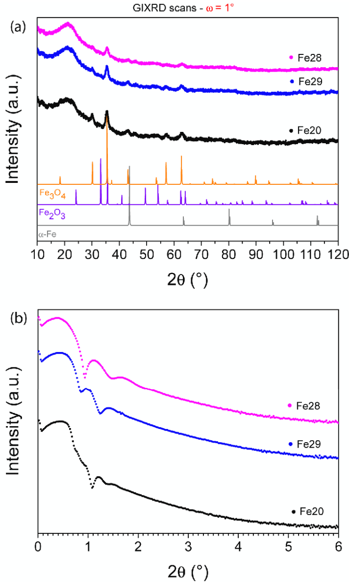
Figure 2. (a) GIXRD (incidence angle \omega=1^\circ ) and (b) XRR experimental scans for the magnetite films reported in table 1. Reference powder diffraction patterns for Fe 3 O 4 , Fe 2 O 3 and \alpha -Fe are also shown.
