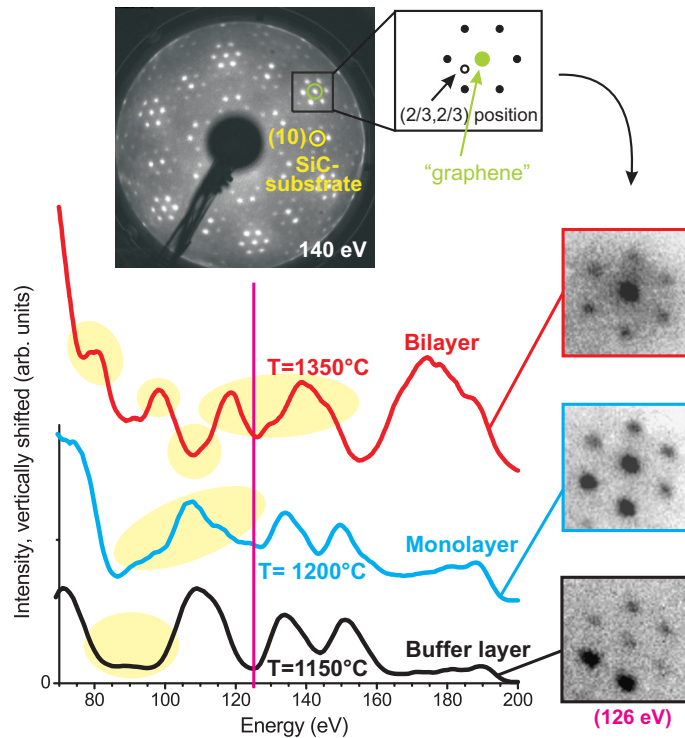
Figure 7. LEED spot intensity spectra for different numbers of epitaxial graphene layers grown (at the indicated temperatures) on 4H-SiC(0001). As indicated in the inset, the spectra were obtained for the green marked spot of the (6\sqrt{3}\times 6\sqrt{3})R30^\circ reconstruction, which is the graphene (10) spot. The first order diffraction spot for the SiC substrate is indicated in the LEED pattern in yellow, the position of the (2/3, 2/3) spot of the (6\sqrt{3}\times 6\sqrt{3})R30^\circ reconstruction in the inset. Yellow patches indicate fingerprint like features in the spectra that allow the unambiguous determination of the number of graphene layers. LEED patterns at 126 eV are shown on the right, also allowing for a discrimination.
