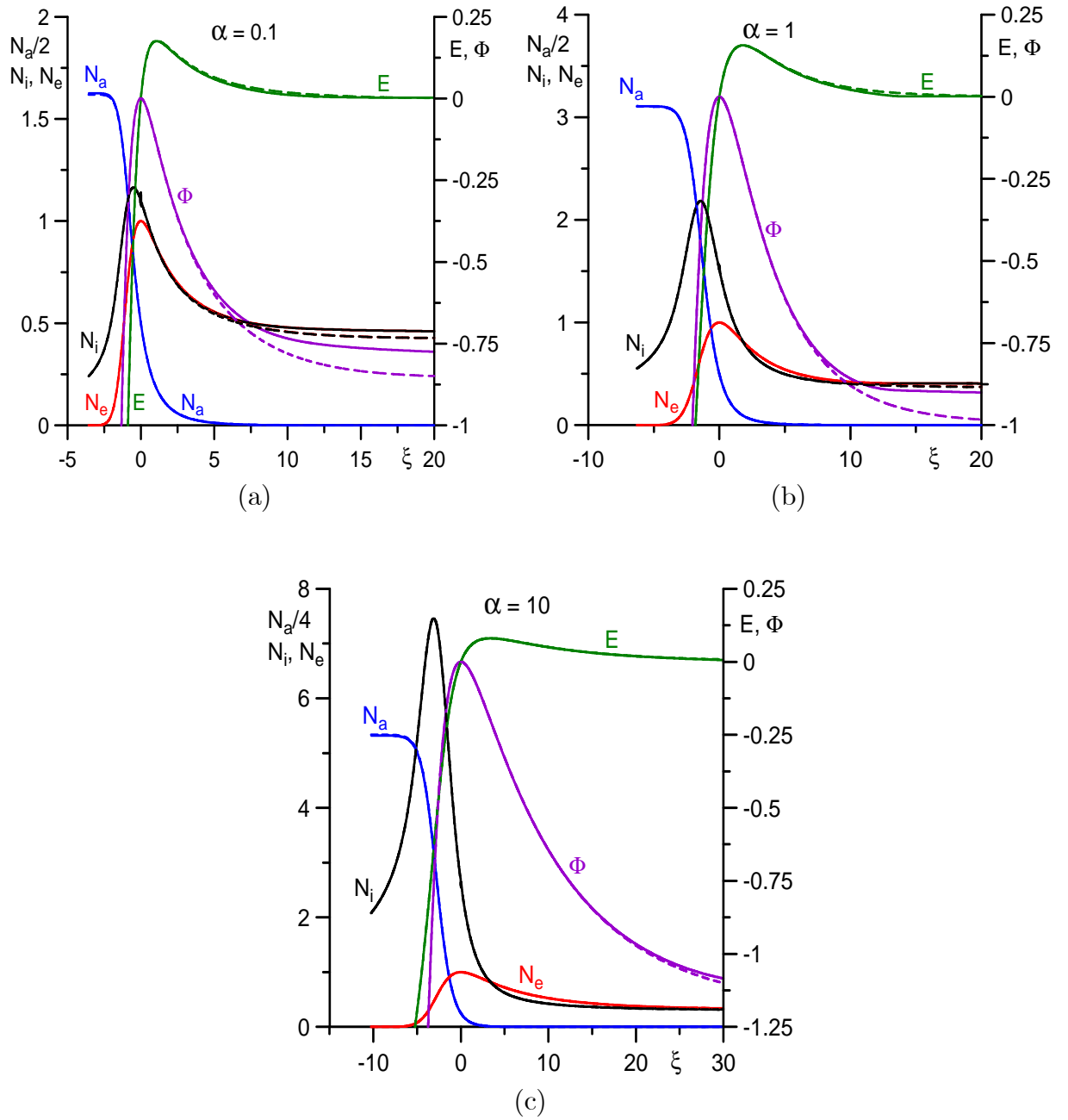
Figure 4. Distribution of parameters across the sheath. Solid: h = 10^{-2} . Dashed: h = 10^{-3} .
