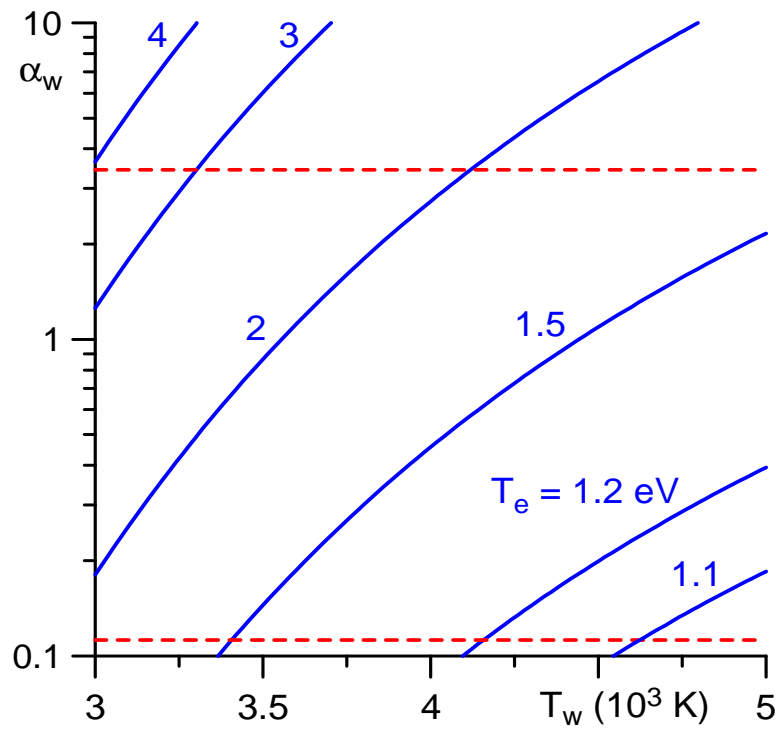
Figure 7. Parameter \alpha_w for a copper cathode.
