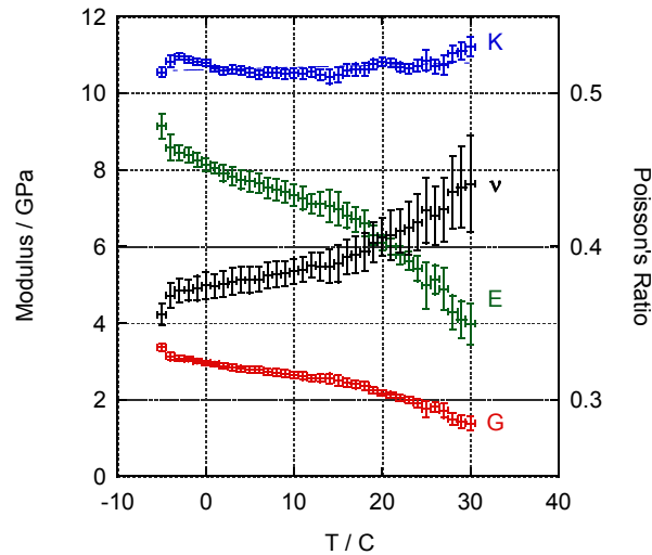
Figure 3. Elastic properties derived from sound speeds, measured using 5 MHz ultrasonic probes.
