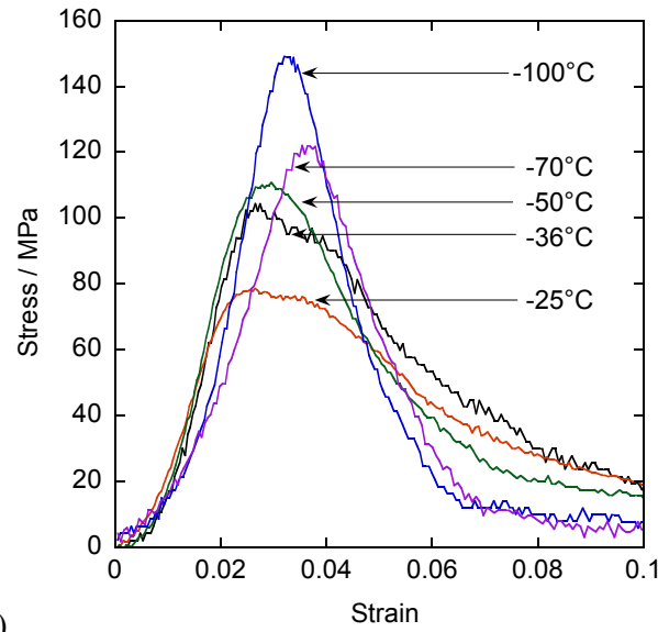
Figure 5. Stress-strain curves for the PBX at nominal strain rates of 2000 \text{ s}^{-1} , across a range of temperatures: (a) 60 to -25^\circ\text{C} (b) -25 to -100^\circ\text{C}
