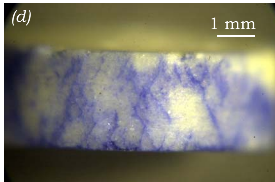
Figure 7. Photographs of PBX specimens (a) undamaged; (b) compressed to 3% strain at -70^{\circ}\text{C} ; (c) compressed to 3% strain at 22^{\circ}\text{C} ; (d) same specimen as figure (c), stained with blue dye to illustrate shear-banding. Scale shown in (a) also applies to (b) and (c).
