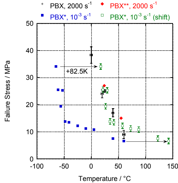
Figure 10. Enlargement of figure 9, with the quasi-static data presented in [5] shifted by \log R = 82.5^\circ\text{C} , where S = 13.1\text{ K} is the shift factor and R = 2 \times 10^6 is the ratio of SHPB to quasi-static strain rates.
