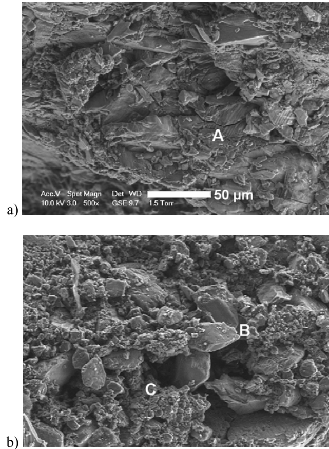
Figure 8. ESEM images showing fracture surfaces of the PBX after recovery from SHPB compression. (a) sub- T_g specimen (0°C) showing crystal fracture at “A”. (b) super- T_g specimen showing a protruding grain at “B” and a recess at “C”, along with less exposed crystal surface than figure 8a, implying adhesive failure. The scale shown in (a) also applies to (b).
