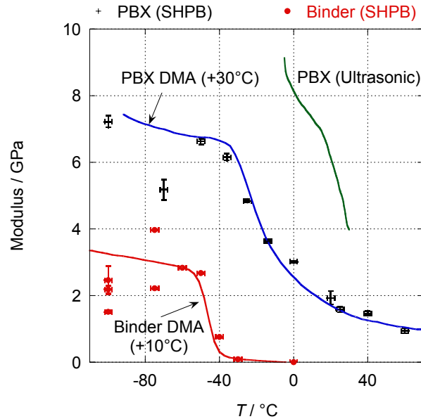
Figure 11. Plot of PBX and Binder “SHPB pseudo-modulus” against temperature, alongside the PBX Young's modulus from figure 3. The DMA curves from figure 1 are included - their modulus values have been re-scaled and temperature-shifted to fit the SHPB moduli shown. The binder DMA required a shift of +10°C and the PBX DMA required a shift of +30°C.
