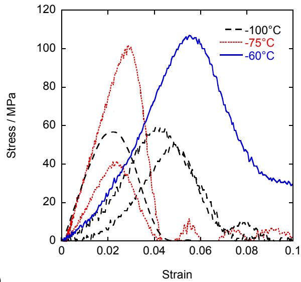
Figure 6. Stress-strain curves for the binder at nominal strain rates of 3000 \text{ s}^{-1} , over a range of temperatures: (a) 0 to -60^\circ\text{C} (b) -60 to -100^\circ\text{C} , including repeats
