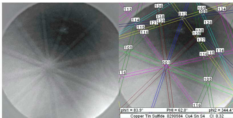
Figure 6. Electron diffraction pattern for the sample sulfurized at 520 °C (C520). The phases and orientations assignment were done using the ICDD database [14].
