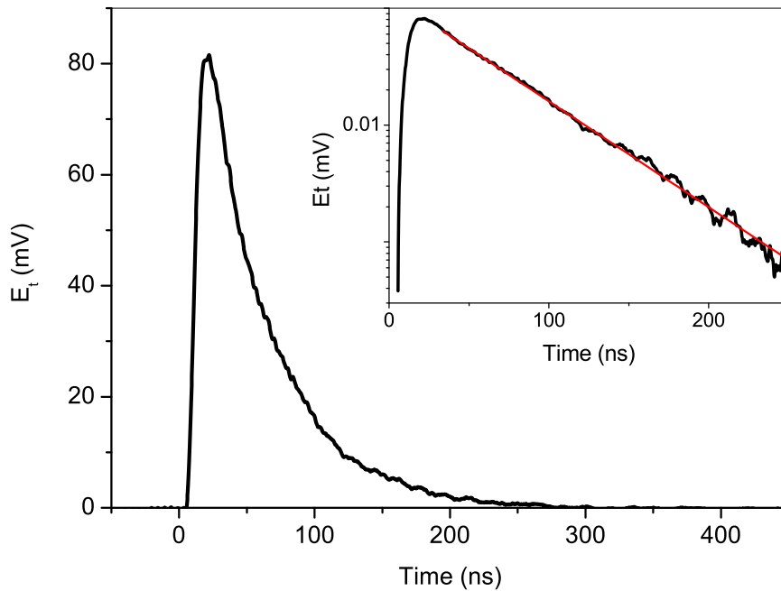
Figure 4. LIF pulse at P= 0.2 Torr, pure N_2 (after background subtraction). The curve shown is the average over 5000 laser shots. The same pulse is shown in logarithmic scale in the inset figure. Single exponential decay starts at about 30 ns, i.e. after about 20-25 ns from the beginning of the pulse. The red line is the exponential fit of the decay.
