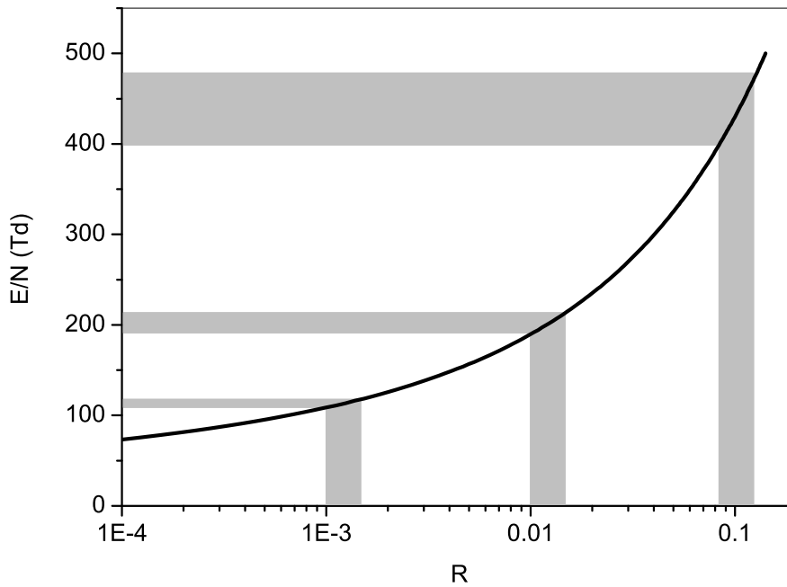
Figure 8. E/N vs. R = r_2/r_1 calculated by BOLSIG+ in pure N_2 . Three uncertainty cases are presented, with R ranging from 10^{-3} to 1.47 \times 10^{-3} , and from 10^{-2} to 1.47 \times 10^{-2} and from 8.3 \times 10^{-2} to 1.23 \times 10^{-1} . The cross sections are taken from [25] and from [26] for processes (1) and (2) respectively.
