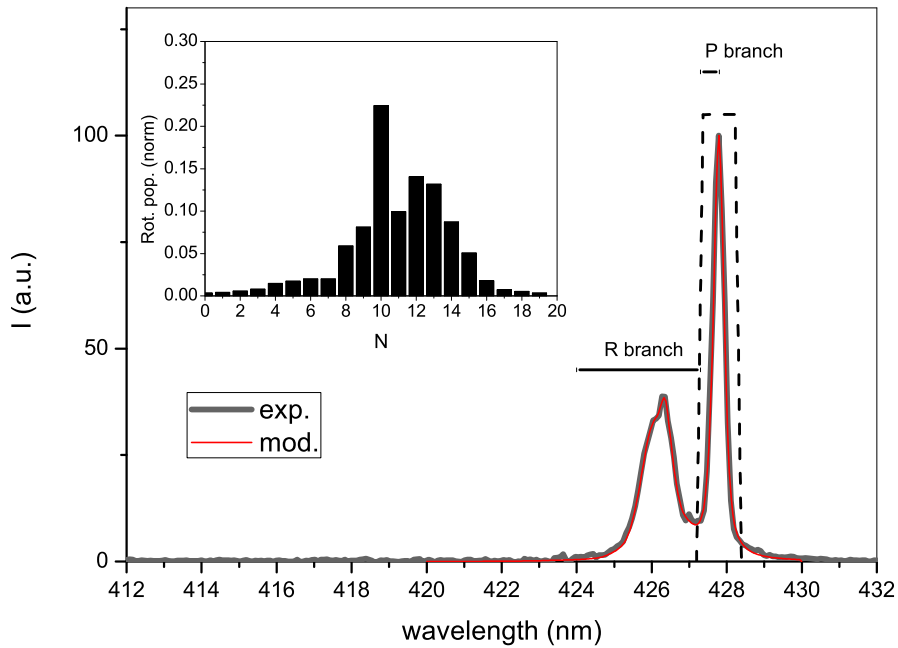
Figure 3. Fluorescence spectrum of FNS (0,1) band after laser excitation at 391.424 nm. The measurement is taken with the ICCD and a bandwidth of about 0.4 nm. The simulation is calculated by LIFBASE and with the rotational populations shown in the inset figure. The dashed lines define the position of the trapezoidal slit spectral transmission function used for LIF pulse measurements.
