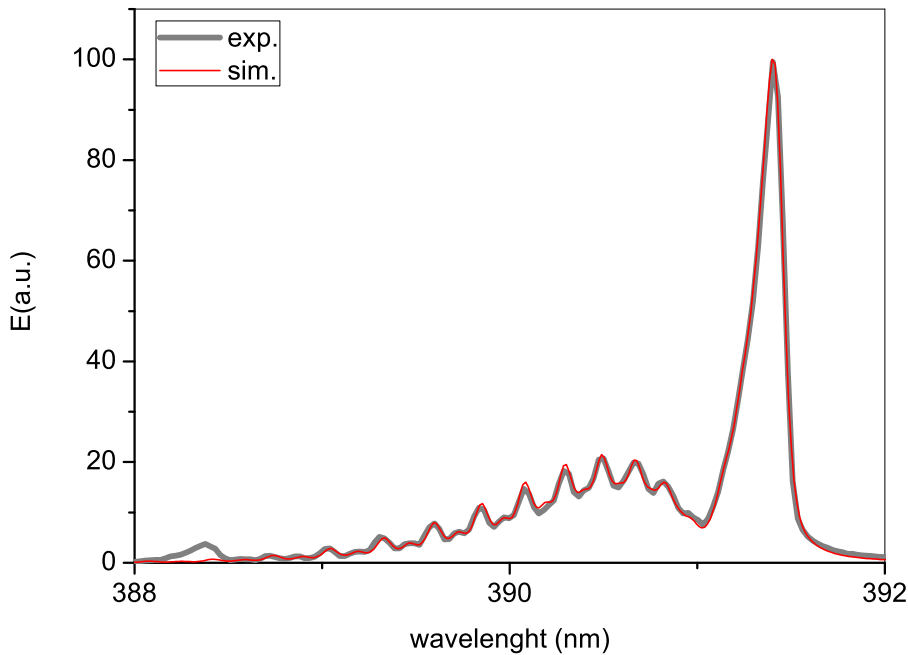
Figure 5. Emission spectrum of FNS (0,0) at 2 Torr of N_2+50\%O_2 . The measurement is taken with the ICCD and the 1800 gr/mm grating, with a gate width of 5 \mu s centered at the time of the laser shot. The simulation is calculated by LIFBASE with a Voigt instrumental profile (gaussian + 50 % Lorentzian), 0.12 nm bandwidth, T_{rot}=330K
