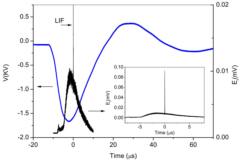
Figure 2. Oscillograms of the applied voltage and FNS (0,1) band emission in N_2 at 2 Torr. The emission scale is compressed in the main figure. In the inset figure the whole emission plus LIF signals are shown in an uncompressed scale.
