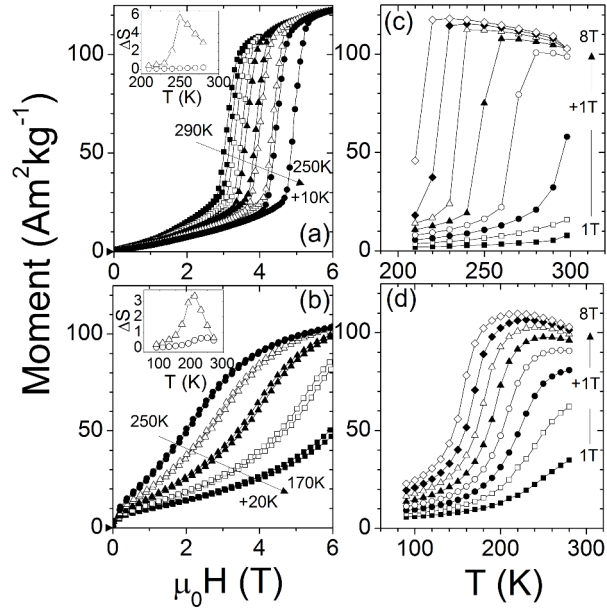
Figure 2. Isothermal M - H loops for a) \text{CoMnSi}_{\text{SC}} at 10K intervals and b) \text{CoMnSi}_{\text{Q}} at 20K intervals. Insets show the entropy change (in units of \text{JK}^{-1}\text{kg}^{-1} ) calculated from this data using the Maxwell relation (Eq. 3) for field changes of 0-2T (open circle) and 0-5T (open triangle). Isofield M - T loops constructed from isothermal magnetization data in magnetic fields at 1T intervals between 1 and 8T for c) \text{CoMnSi}_{\text{SC}} and d) \text{CoMnSi}_{\text{Q}} .
