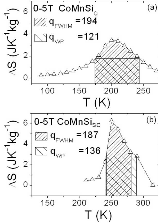
Figure 8. Refrigerant capacity calculated using the FWHM (dense shading) and Wood & Potter method (sparse shading) with a field change of 0-5T for a) \text{CoMnSi}_Q and b) \text{CoMnSi}_{SC} .
