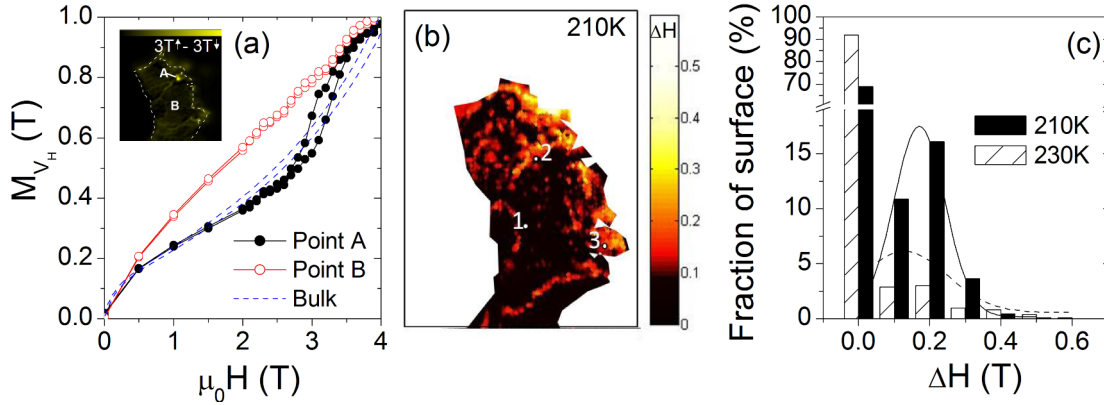
Figure 6. (Colour online) Hall probe imaging of \text{CoMnSiQ} . a) Local M - H loops constructed from data taken for a single pixel at the two points marked A and B on the difference image (inset). The global M - H loop taken from the bulk sample at this temperature is also shown, normalized to M=1 at 4\text{T} , where the colour scale is fixed, with white (yellow online) corresponding to a large difference in moment, i.e. finite hysteresis, and black to zero or negligible difference in moment ( \Delta H=0 ). (b) Map of the hysteresis observed by Hall probe imaging at 210\text{K} . The colour scale indicates the magnitude of hysteresis where black (red online) for \Delta H = 0 and white for \Delta H > 0.4 . Points 1, 2 & 3 indicate areas that were investigated with EDX to check if there was some variation in stoichiometry associated with the change of magnetic behaviour. c) Statistical distribution of hysteresis, \Delta H , measured for single pixels across the sample surface during Hall Probe imaging at 210 and 230\text{K} . A Gaussian fit for this data (ignoring \Delta H = 0 ) is indicated by the dotted and solid lines for 230 and 210\text{K} respectively.
