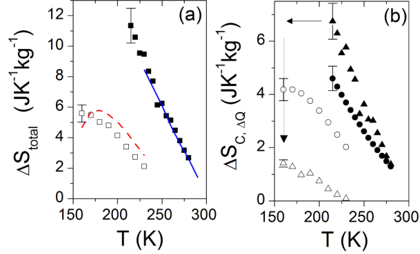
Figure 4. (Colour online) a) Total isothermal entropy change of CoMnSi SC (closed symbols) and CoMnSi Q (open symbols) for small fragments measured by calorimetry compared with \Delta S_M derived from bulk magnetization measurements (-,---), b) Separate contributions to the entropy change, \Delta S_{HC} (circles) & \Delta S_{LH} (triangles), for CoMnSi SC (closed symbol) and CoMnSi Q (open symbol). The arrow indicates the reduction in latent heat at equivalent AFM-FM transition temperatures. All data in (a) & (b) is for a field change of 0-8T and the level of error is indicated by the error bars on the first data point (<10%).
