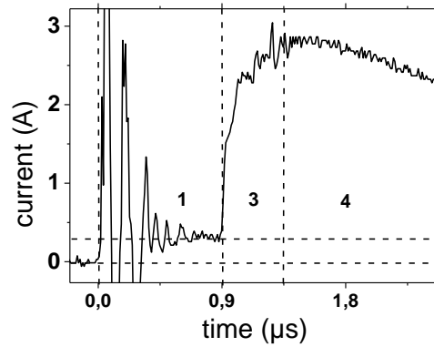
Figure 4c. Current waveform in 500 \mu S/cm water, there is no reillumination spikes, (1) initiation current, (3) propagation, (4) decay, there is a large current even when the discharge has stopped to propagate and just decay according to the voltage pulse decay, (4cm gap, 40kV).
