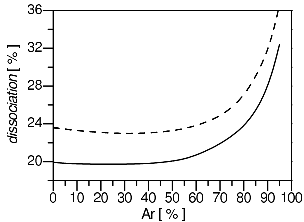
Figure 13. Dissociation degree for two different tube radius: 0.25 cm (—) and 0.5 cm (---), at 2 Torr .
