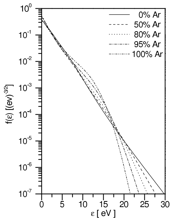
Figure 5. Self-consistent EEDFs calculated at p = 2 Torr, for different Ar content in the mixture.
