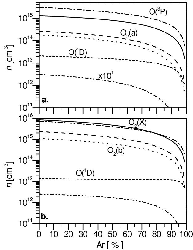
Figure 11. Density of the different oxygen species as a function of Ar percentage in the Ar-O 2 mixture, at 0.5 Torr (a) and at 2 Torr (b): O 2 (X) (—), O 2 (a) (— — —), O 2 (b) (· · · · ·), O( 3 P) (— · —), O( 1 D) (— — —), O 3 (— · · —).
