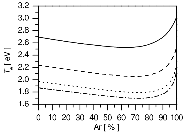
Figure 6. Electron kinetic temperature, T_e = (2/3)\langle\varepsilon\rangle , as a function of the mixture composition, for different values of pressure: 0.5 Torr (—), 1 Torr (— — —), 2 Torr (·····), 3 Torr (— · —).
