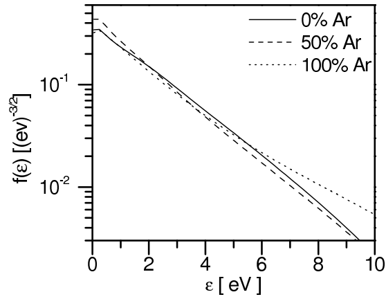
Figure 7. Zoom of figure Figure 5 for \varepsilon < 10 eV.
