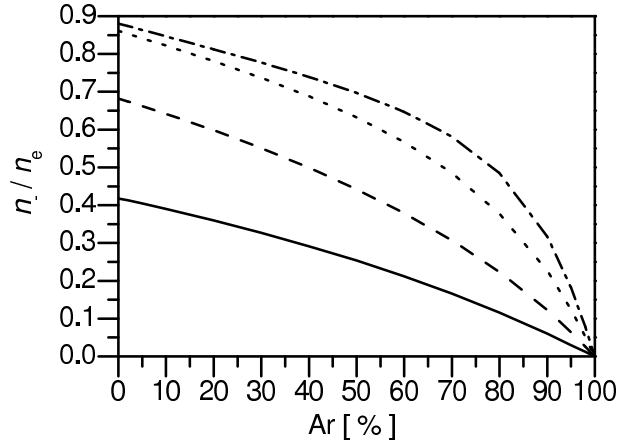
Figure 9. Electronegativity as a function of the mixture composition at different pressures: 0.5 Torr (—), 1 Torr (---), 2 Torr (·····), 3 Torr (- · -).
