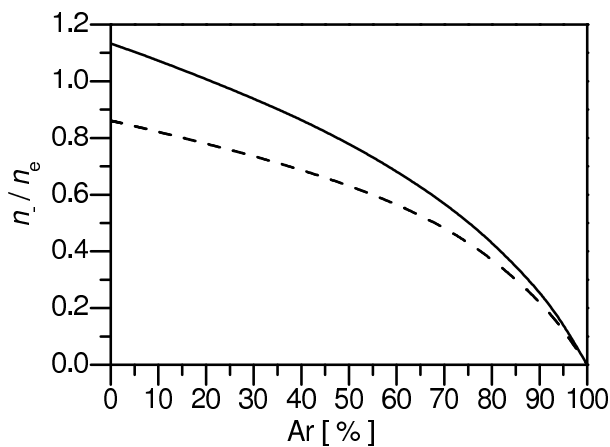
Figure 14. Electronegativity for two different tube radius: 0.25 cm (—) and 0.5 cm (---), at 2 Torr .
