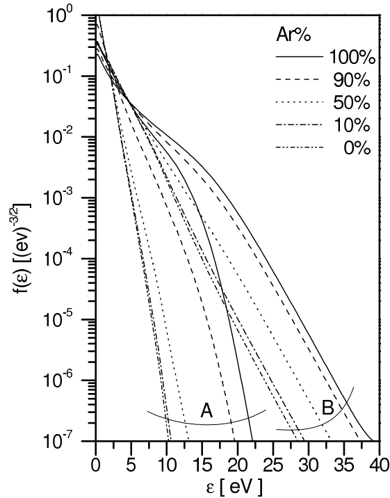
Figure 2. Electron Energy Distribution Function at 150 Td (A) and 550 Td (B) for different Ar-O 2 mixture compositions at 2 Torr with [O]/[O 2 ]=1.
