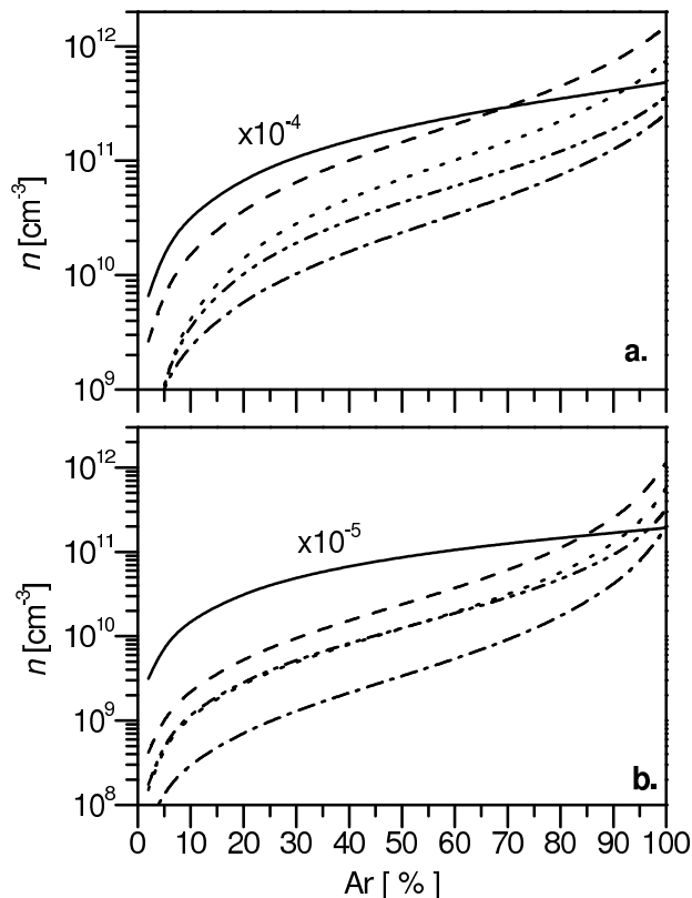
Figure 10. Density of the different Ar atomic states as a function of Ar percentage in the Ar-O 2 mixture, at 0.5 Torr (a) and at 2 Torr (b): Ar( 1 S 0 ) (—), Ar( 3 P 2 ) (---), Ar( 3 P 1 ) (·····), Ar( 3 P 0 ) (— · —), Ar( 1 P 1 ) (— · · —).
