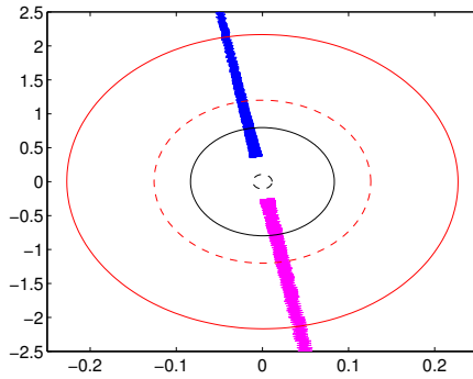
Figure 8: Trajectories in the state-space and attracting sets for N = 1 and N = 8 in case of uncertainties
