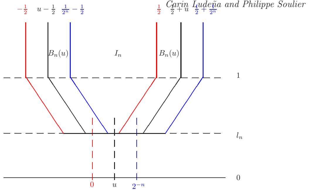
Figure 2. The sets I_n and B_n(u)
