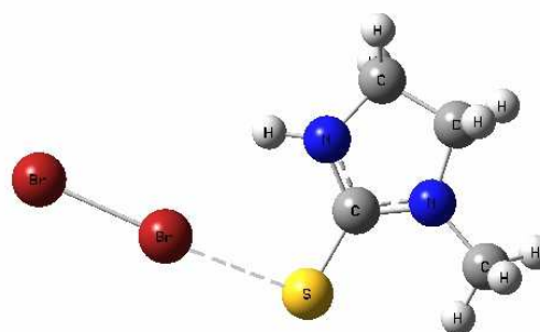
M'-Br-Br planar
