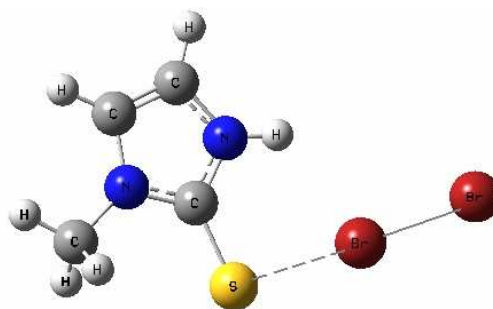
M-Br-Br planar
