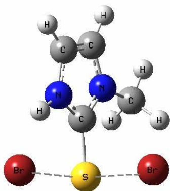
MBr 2 T-shaped
