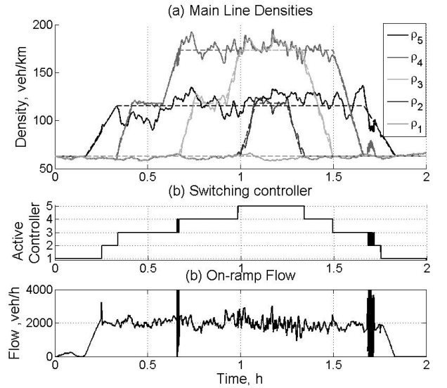
Fig. 9. Switching PI controller
